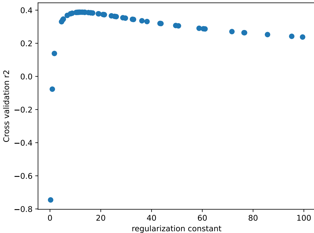
Influence of the regularization parameter on the validation R2 score test R2: 0.402
