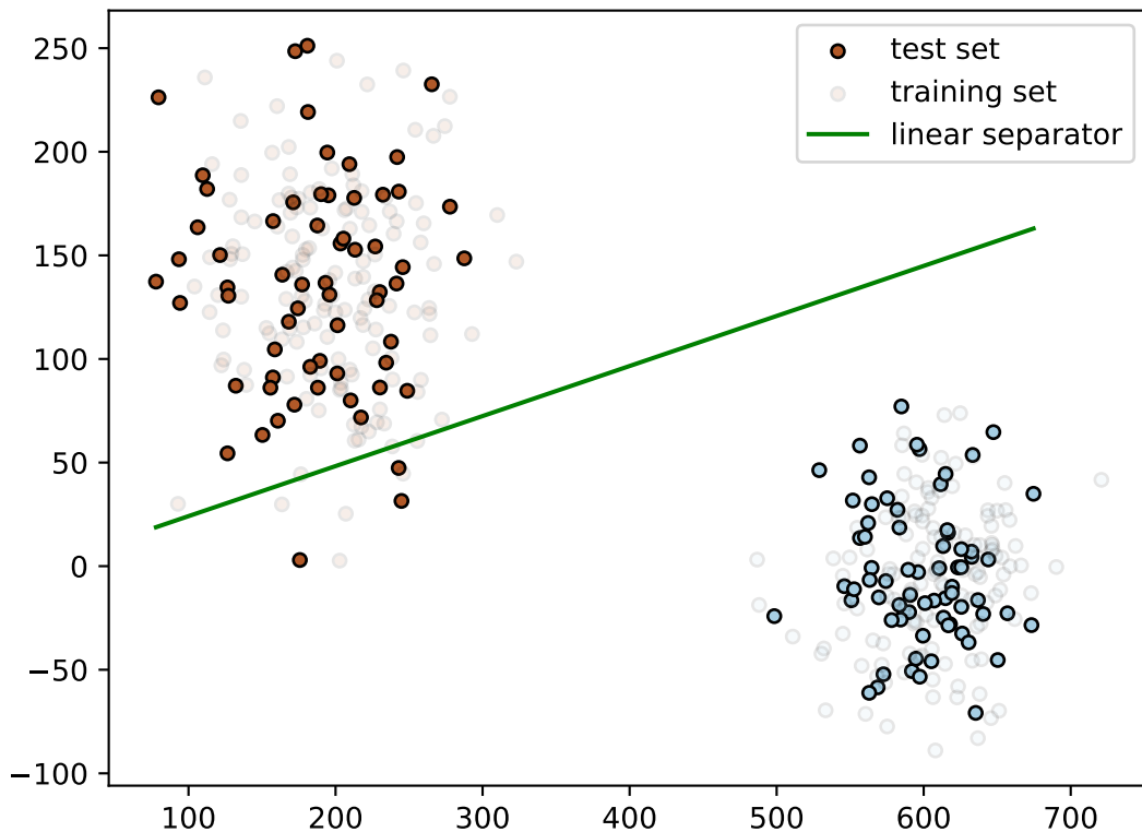
dataset_1 without_standardization score on test set 97.73 %
