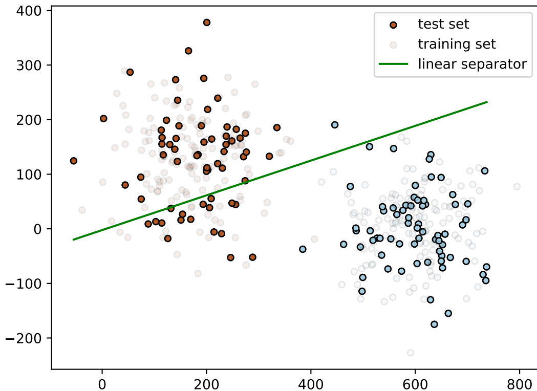
dataset_2 without_standardization score on test set 86.36 %
