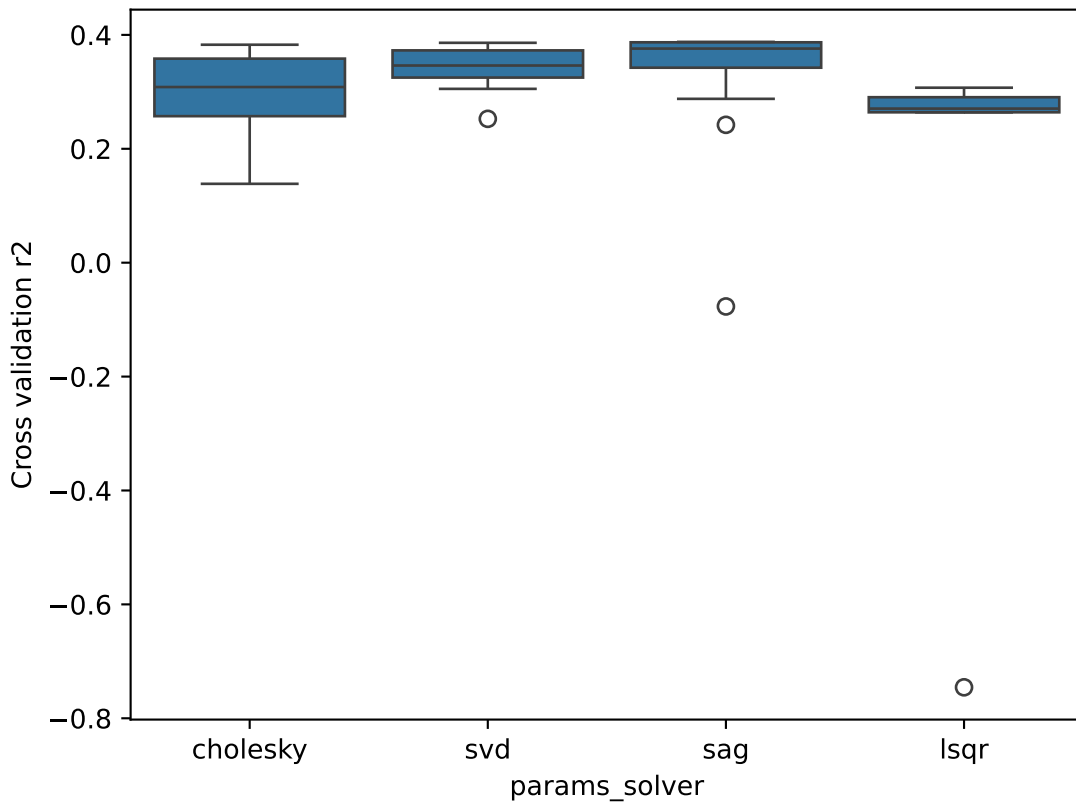
influence of the solver on the validation R2 score test R2: 0.402
