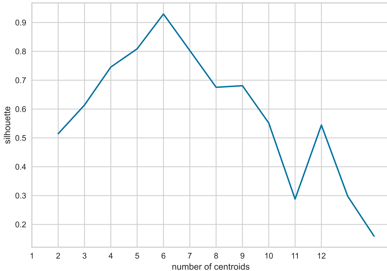
Silhouette score as a function as the number of centroids
