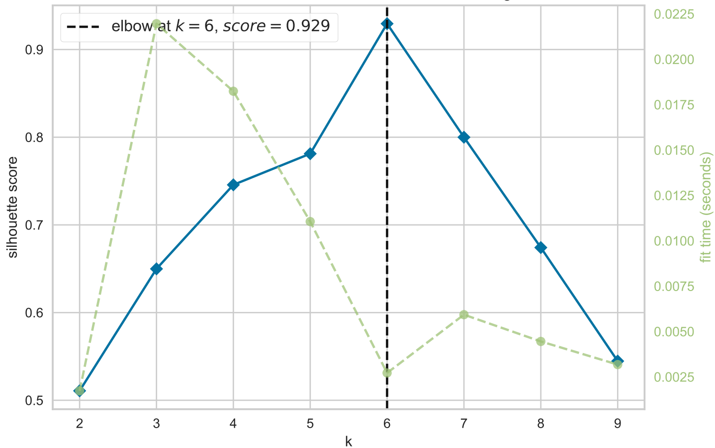
Silhouette Score Elbow for KMeans Clustering
