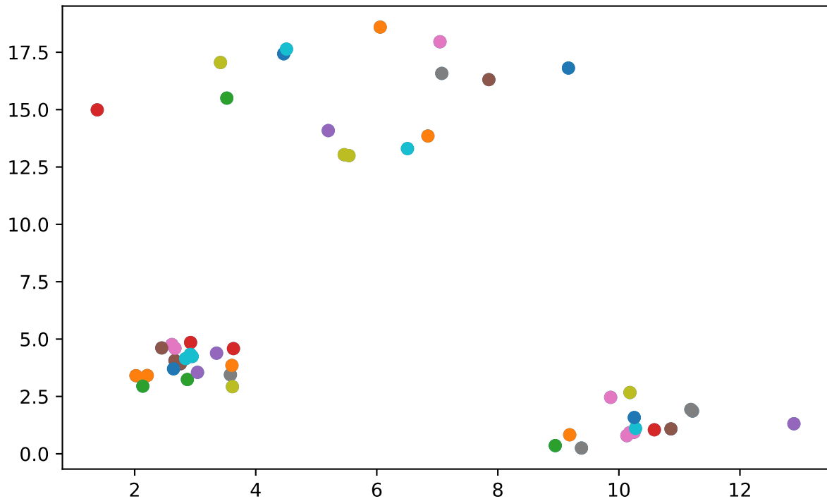
hierarchical clustering step 9 41 clusters euclidean metric
