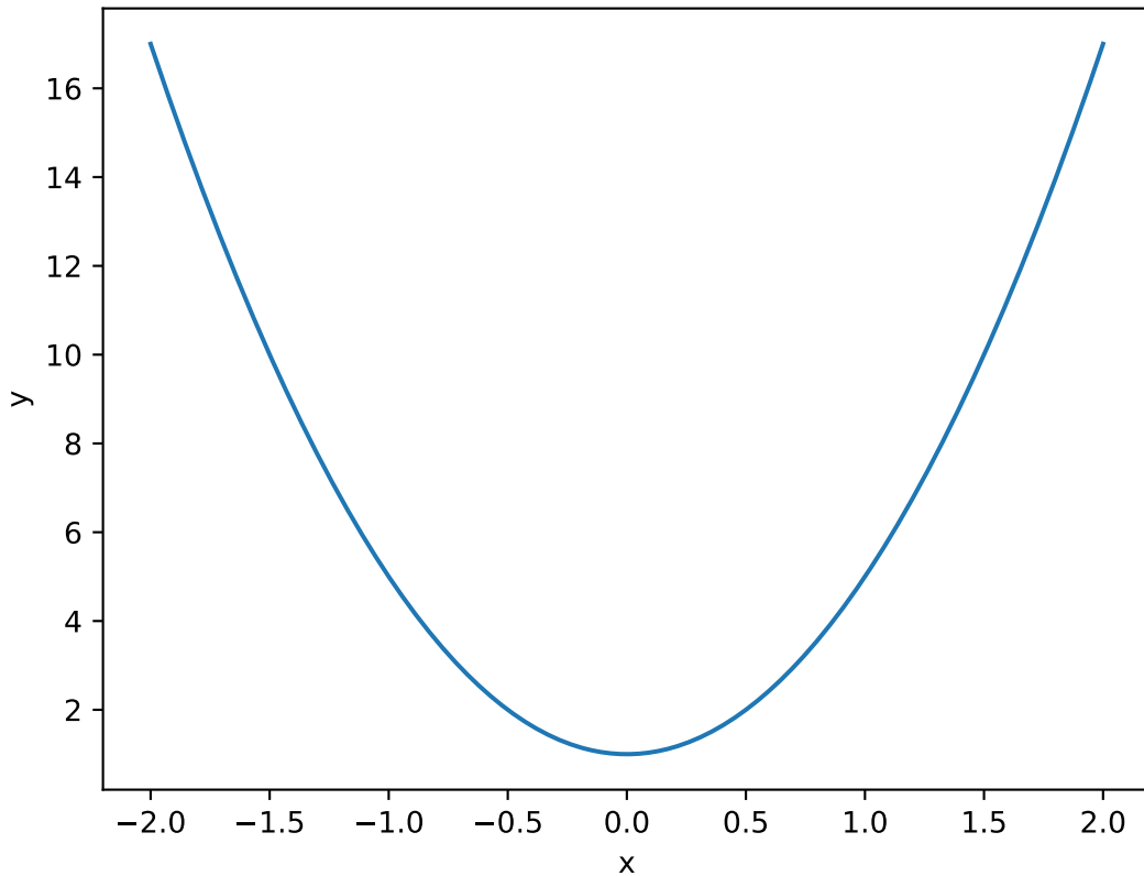
convex function
