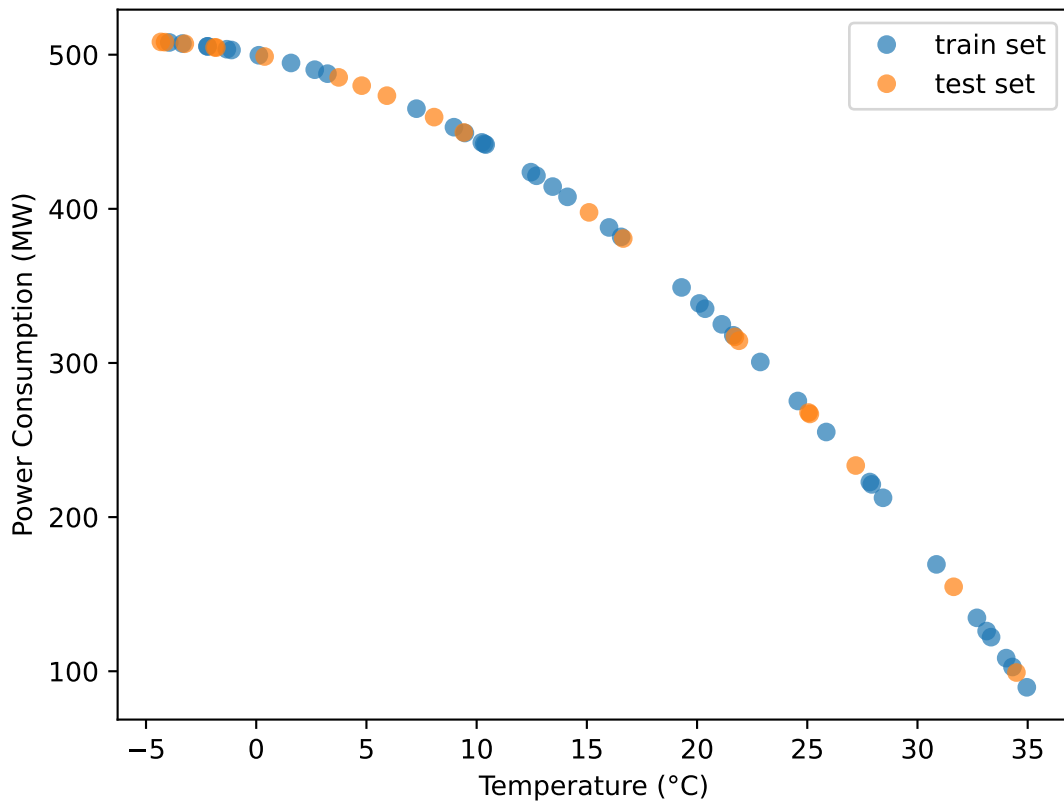
Temperature (°C) vs power consumption (MW) noise standard deviation 0.0
