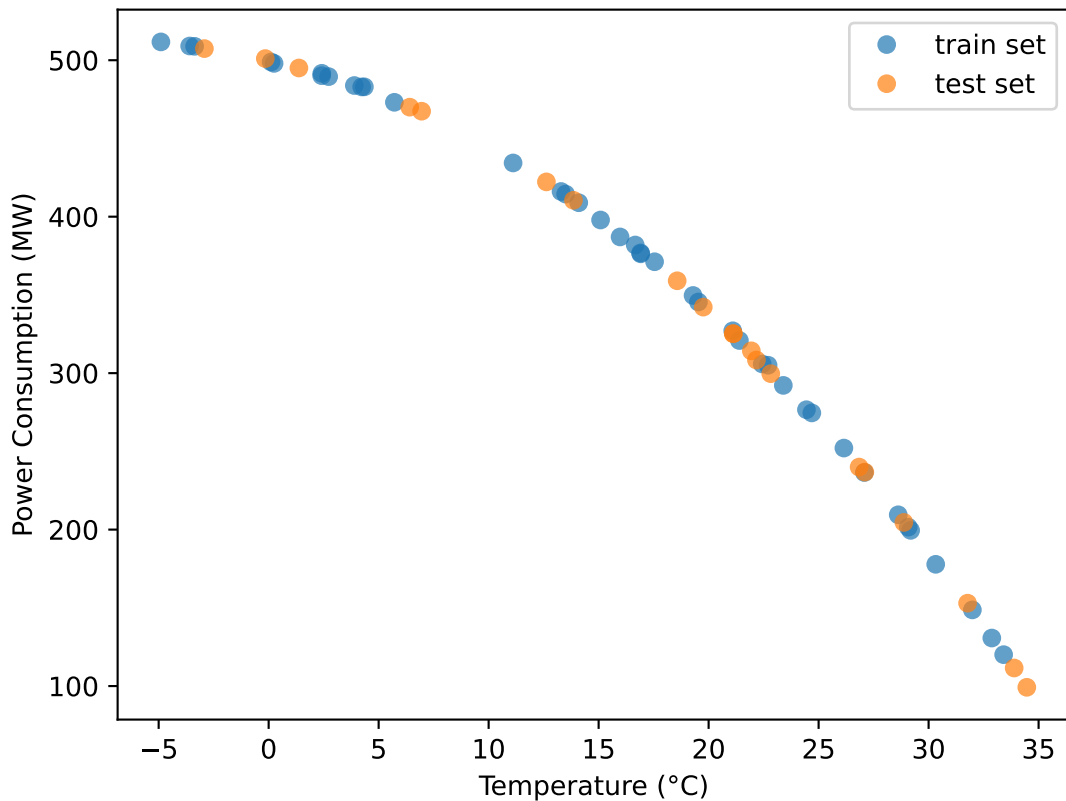
Temperature ( ^{\circ}\text{C} ) vs power consumption (MW) noise standard deviation 1.0
