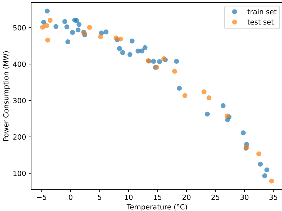
Temperature ( ^{\circ}\text{C} ) vs power consumption (MW) noise standard deviation 20.0
