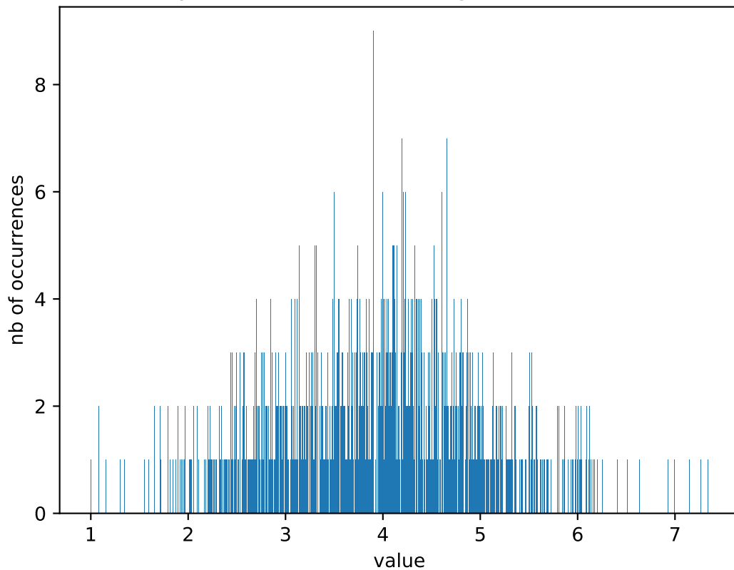
mysterious distro 1 : histogram, 1000 bins
