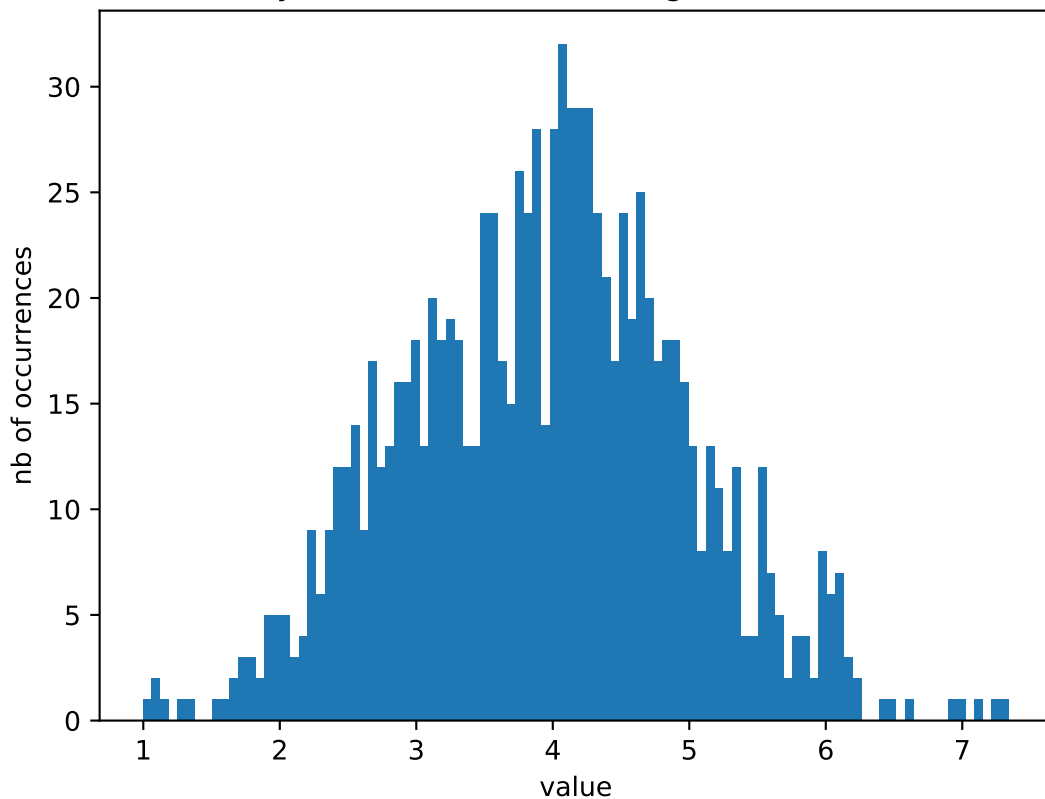
mysterious distro 1 : histogram, 100 bins
