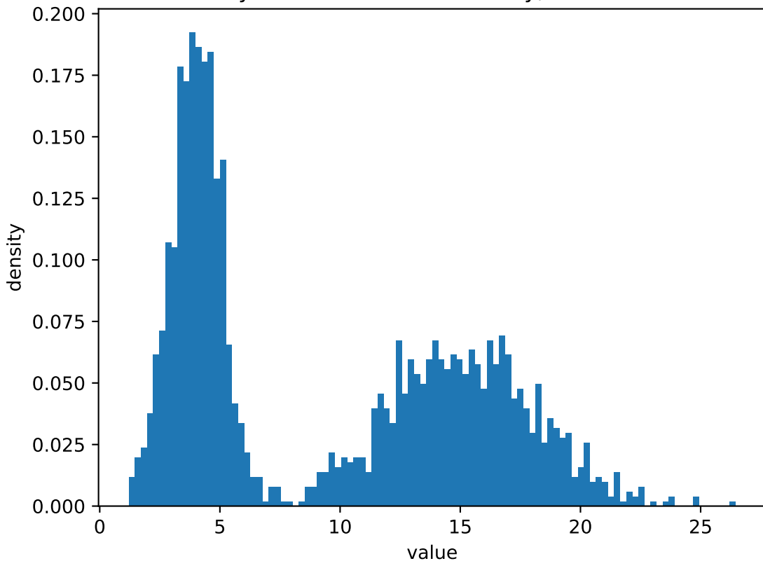
mysterious distro 2 : density, 100 bins
