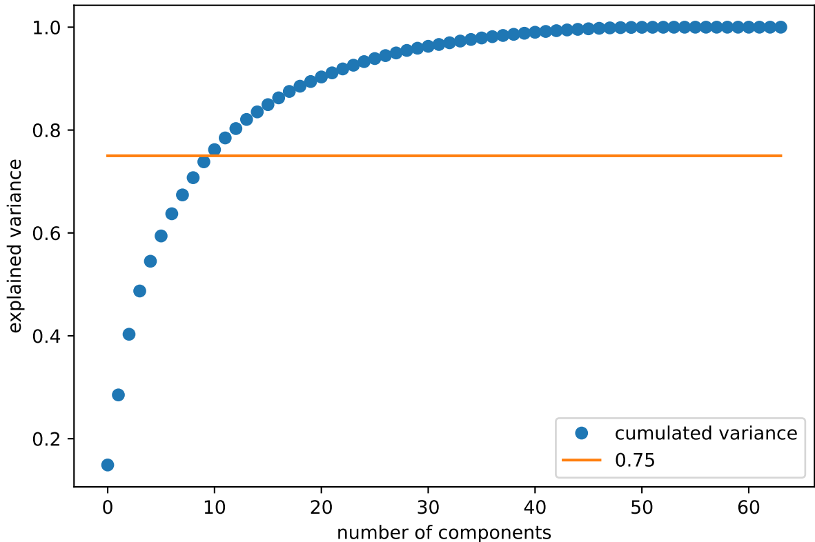
Cumulated variance 76.195% of variance kept with 10/64 components
