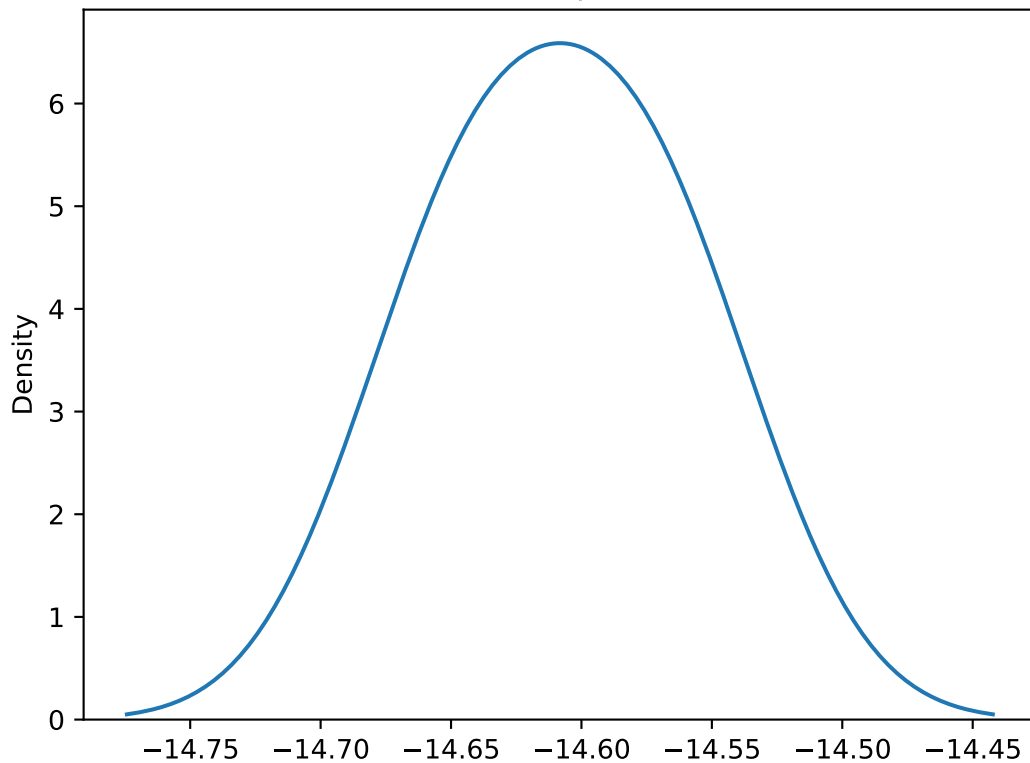
kernel density estimation 1 samples
