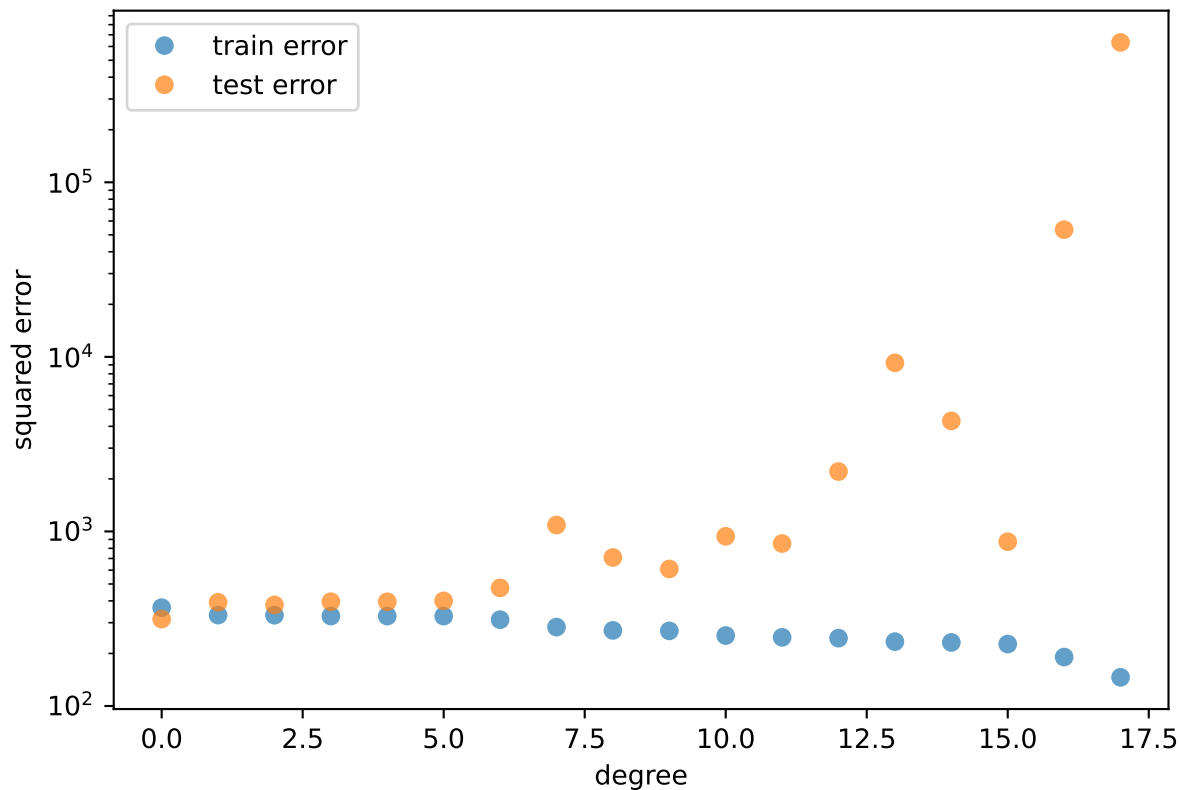
Polynomial regression noise standard deviation 20.0
