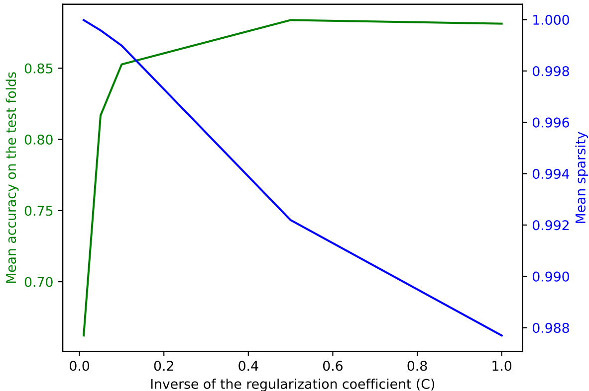
Sparsity and cross-validated accuracy of a logistic regression with L1 penalty
