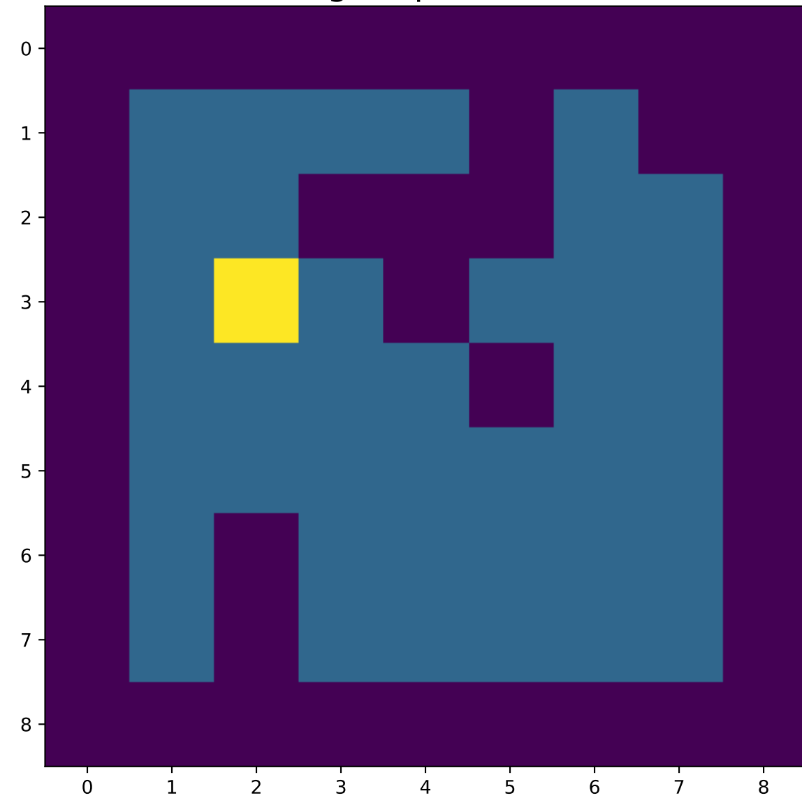
Agent position
