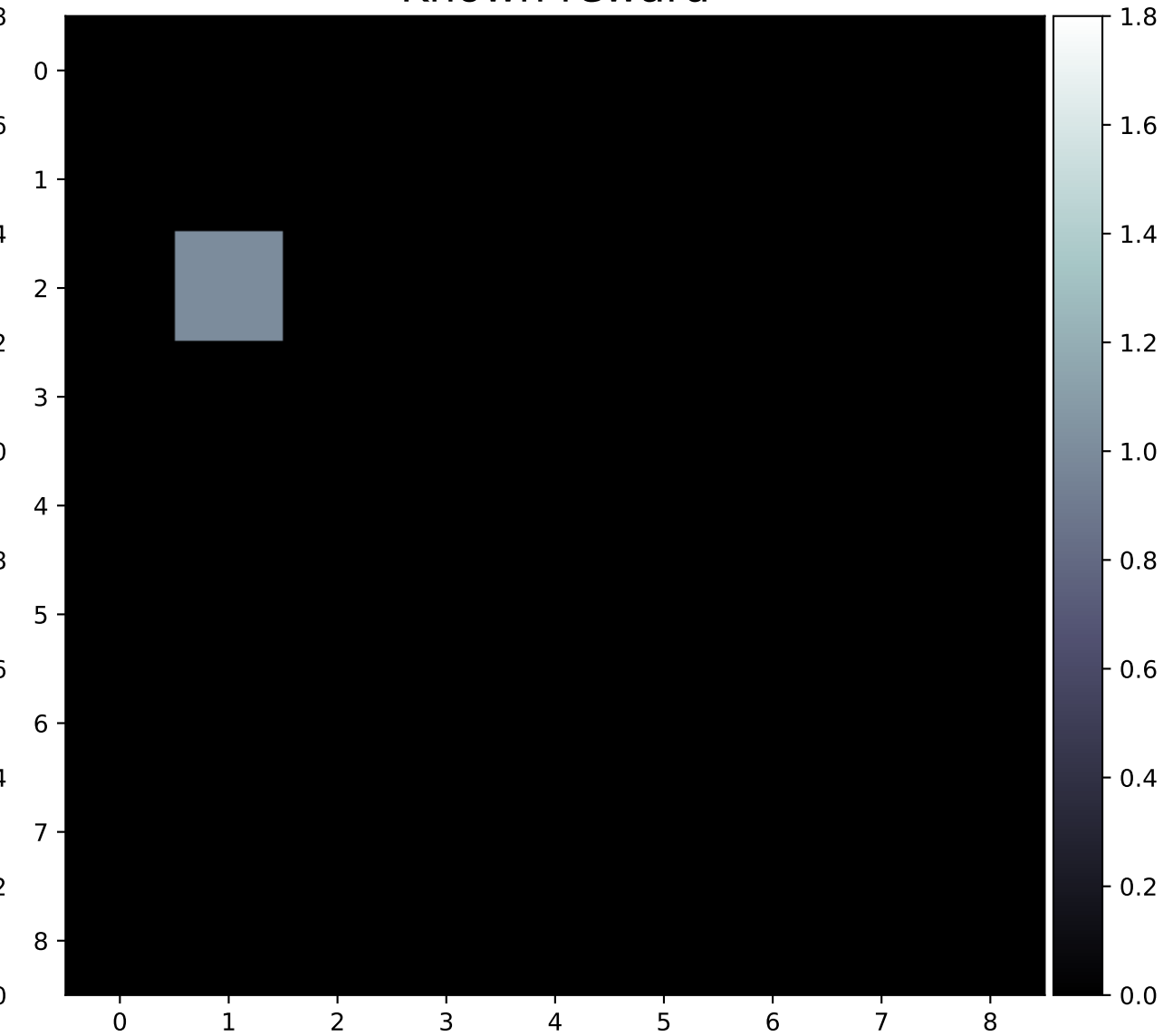
Known reward
