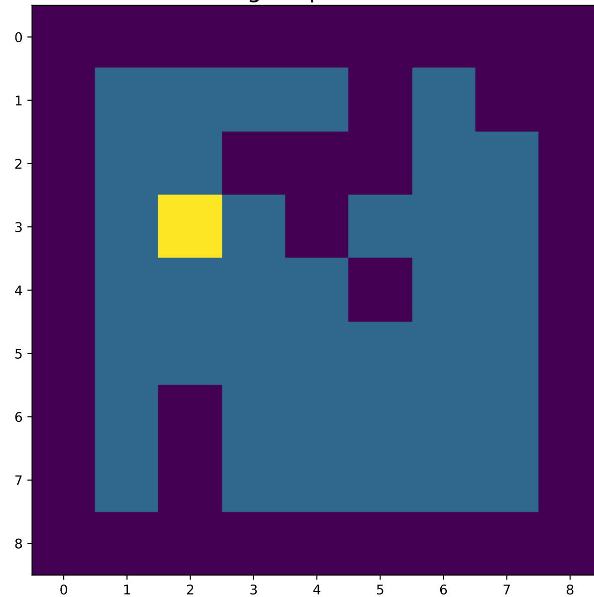
Agent position
