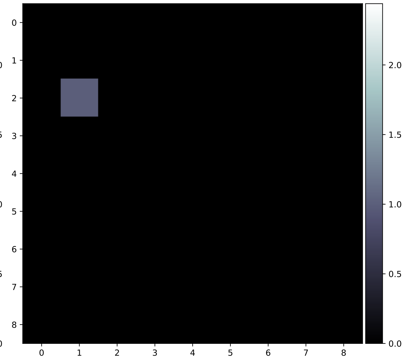
Known reward
