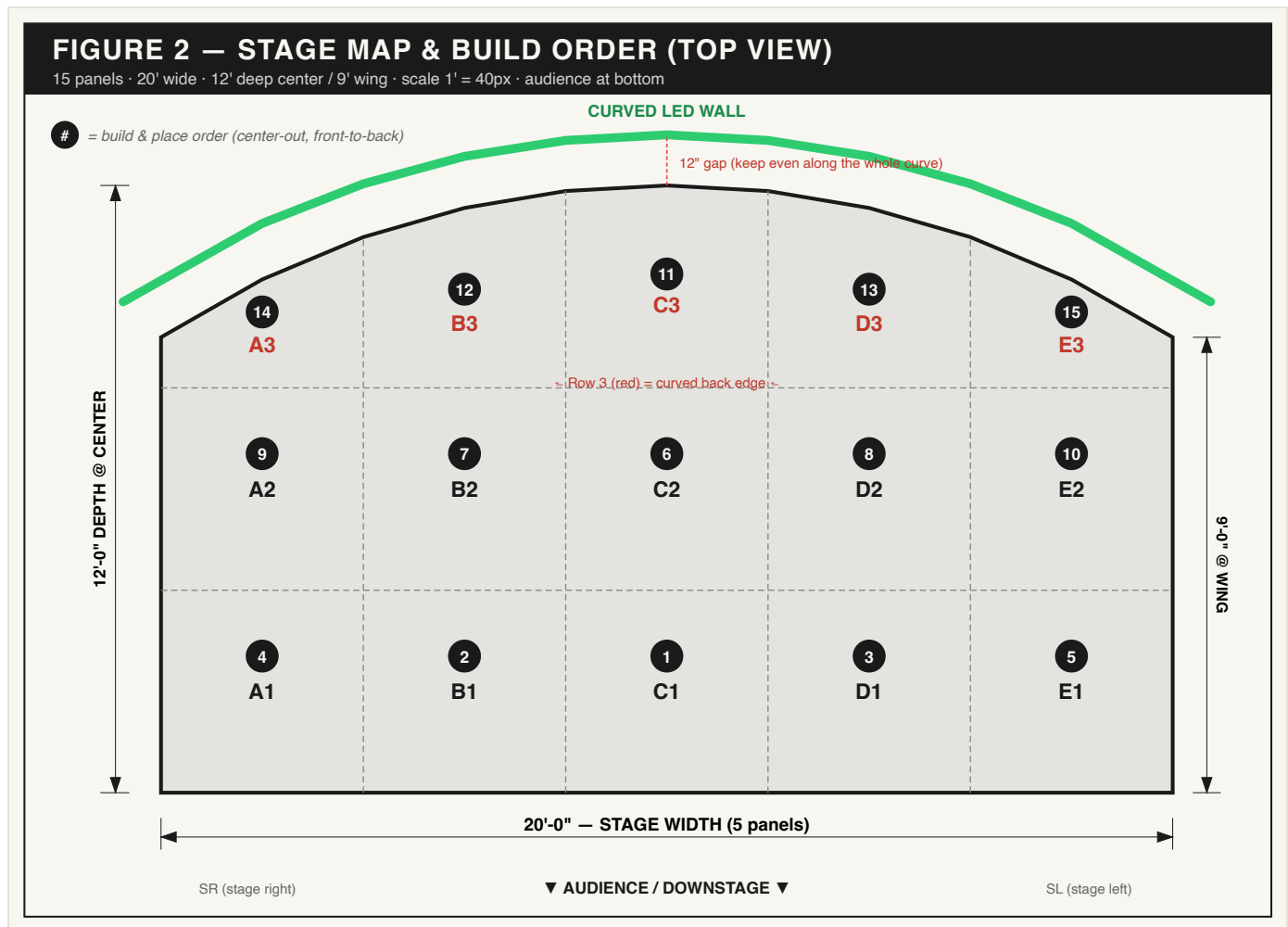
Figure 2 — Top-down map. Build and place panels in the numbered order. The back row (3) follows the LED-wall arc.
