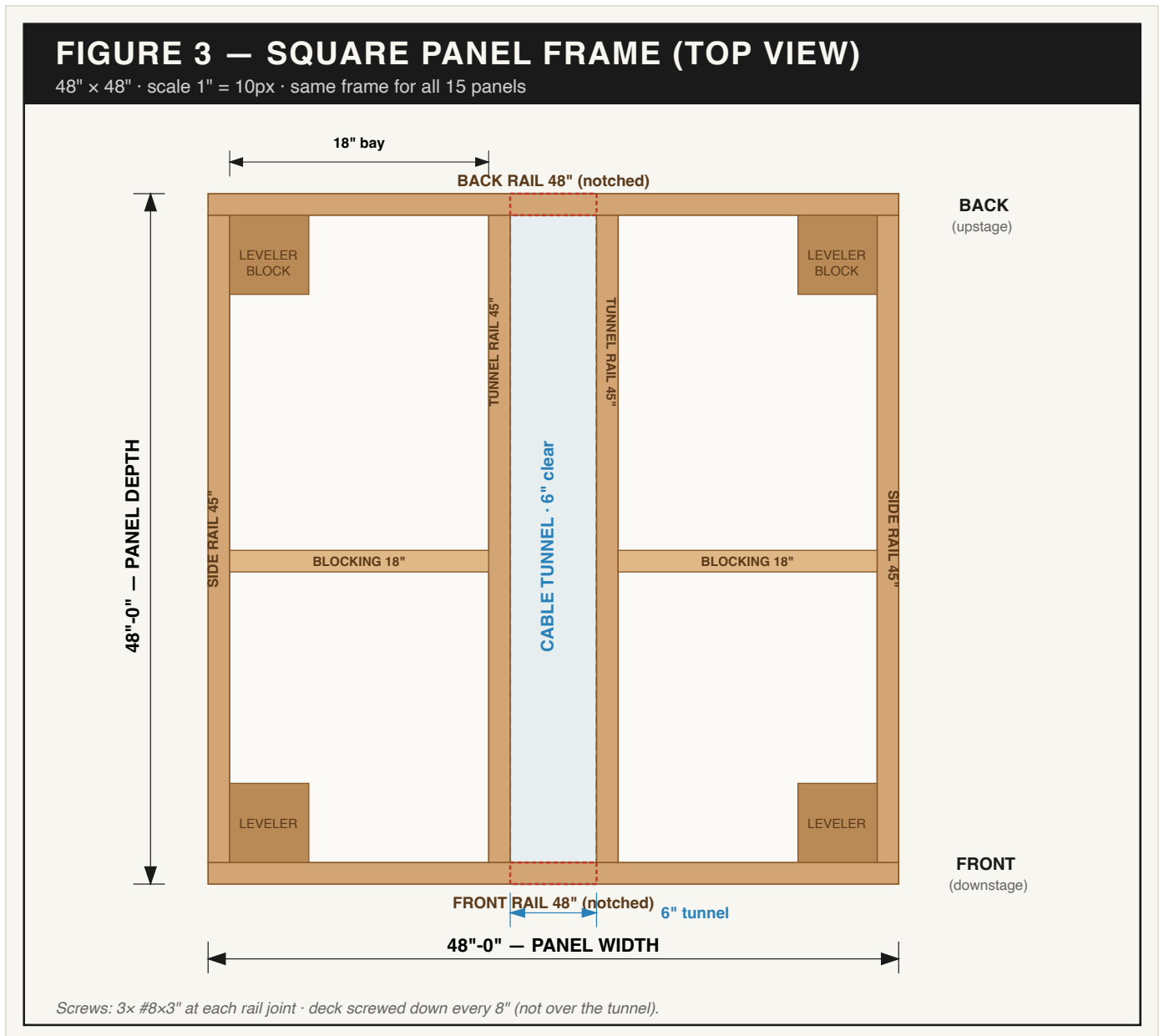
Figure 3 — Square panel frame, seen from above. All inside measurements are clear-gap dimensions.
