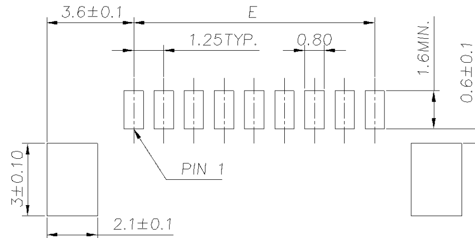
PCB LAYOUT FOR SURFACE MOUNTING (TOP VIEW) (TOLERANCE: ±0.05MM)
