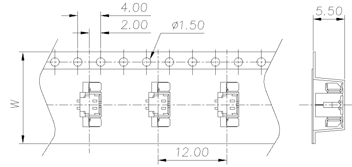
CARRIER FOR 2 TO 7 PIN
