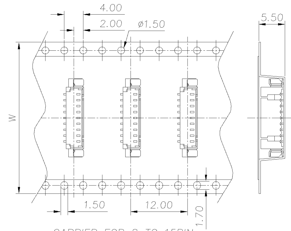
CARRIER FOR 8 TO 15PIN
