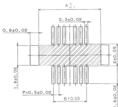
■DF12N with metal fitting
