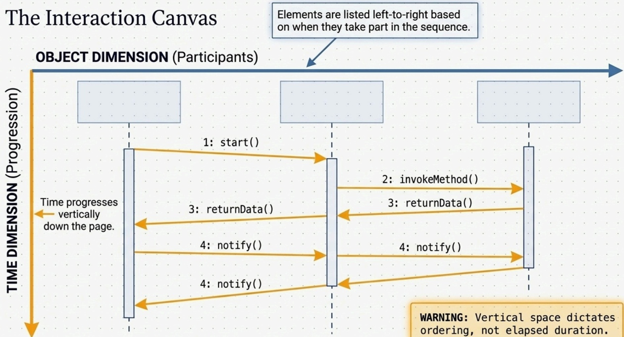
Figure 4.5.2: The Two-Dimensional Interaction Canvas. The horizontal axis organizes participating object lifelines; the vertical axis represents the irreversible passage of time descending downwards.
