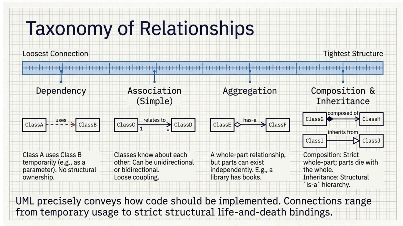
Figure 4.4.4: Taxonomy of Class Relationships. Showing the hierarchy from loose, transient dependencies to tight, permanent lifecycle bindings.
