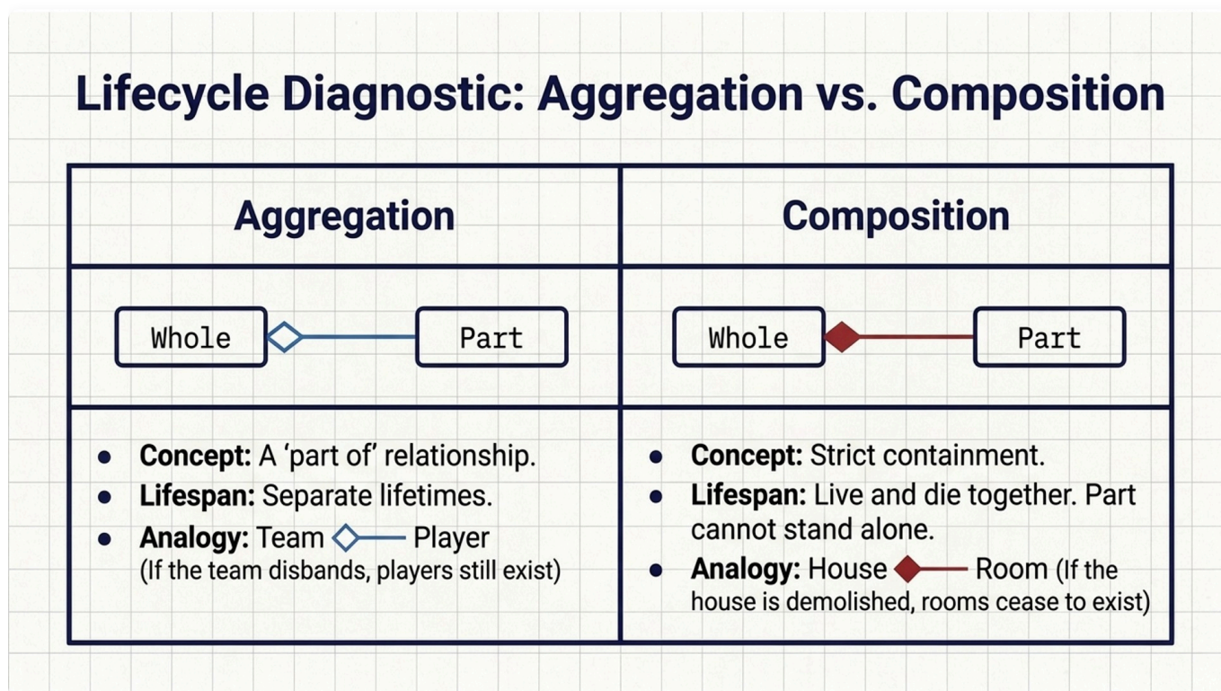
Figure 4.4.6: Aggregation vs. Composition. The definitive test is lifecycle dependency: if the container object is deleted, do the contained objects cease to exist?
