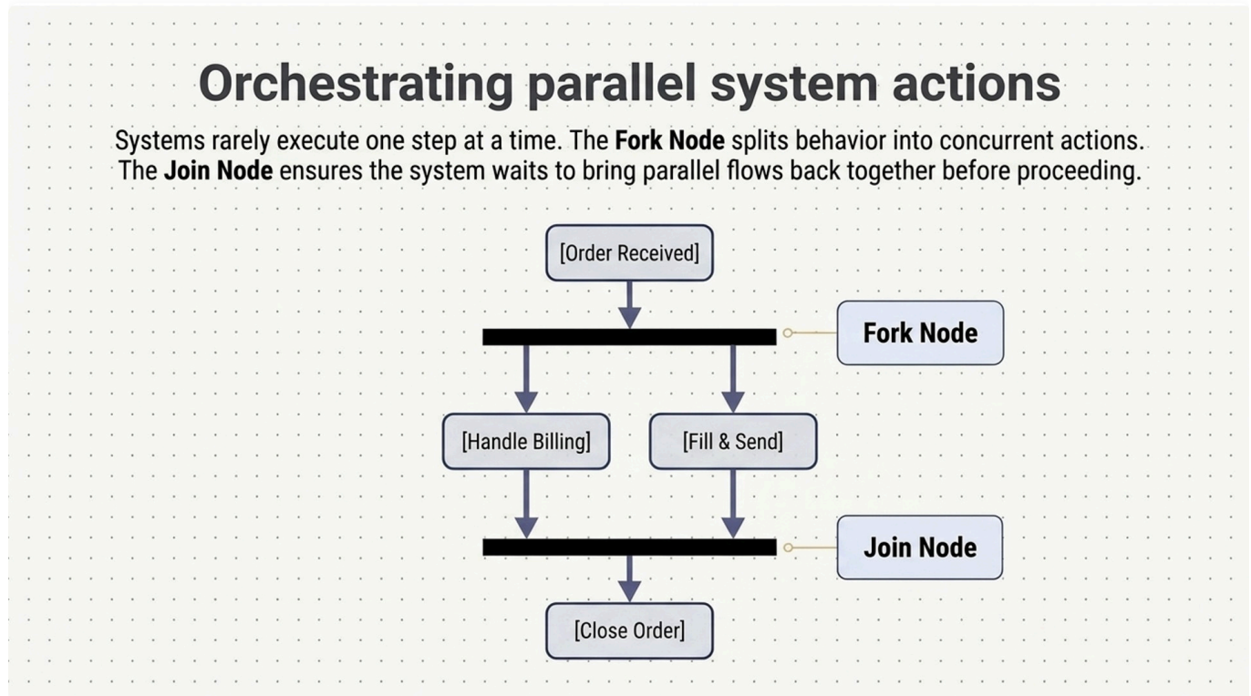
Figure 4.6.3: Concurrency Synchronization with Fork and Join. A Fork node splits a single incoming token into multiple parallel concurrent flows; a Join node synchronizes them back into one.
