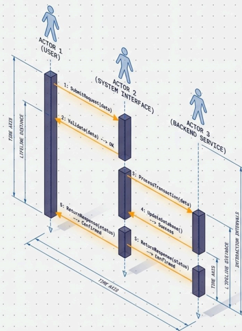
Figure 4.5.1: Dynamic Interaction Overview. Contrasting static class structures with dynamic, time-ordered runtime message exchanges.
