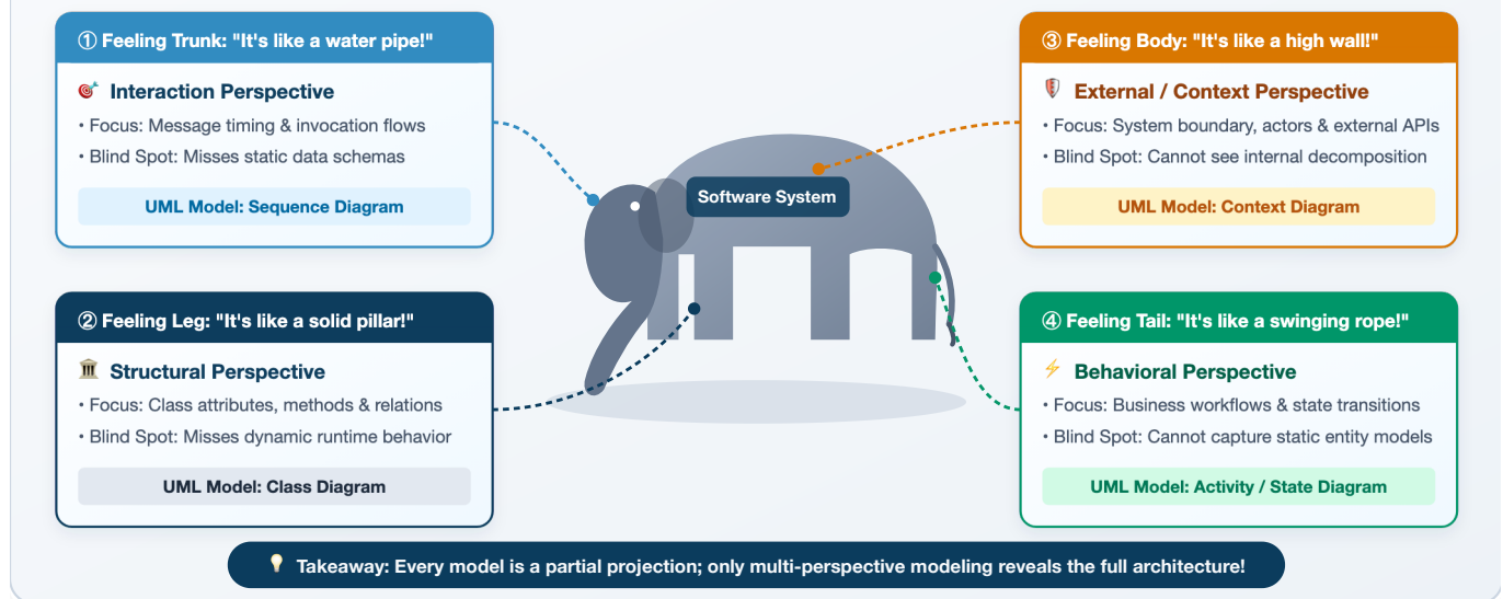
Figure 4.1.1: The Blind Men and the Elephant Metaphor. Just as each observer experiences only one facet of the elephant, each UML diagram captures a specific perspective of the system architecture.
