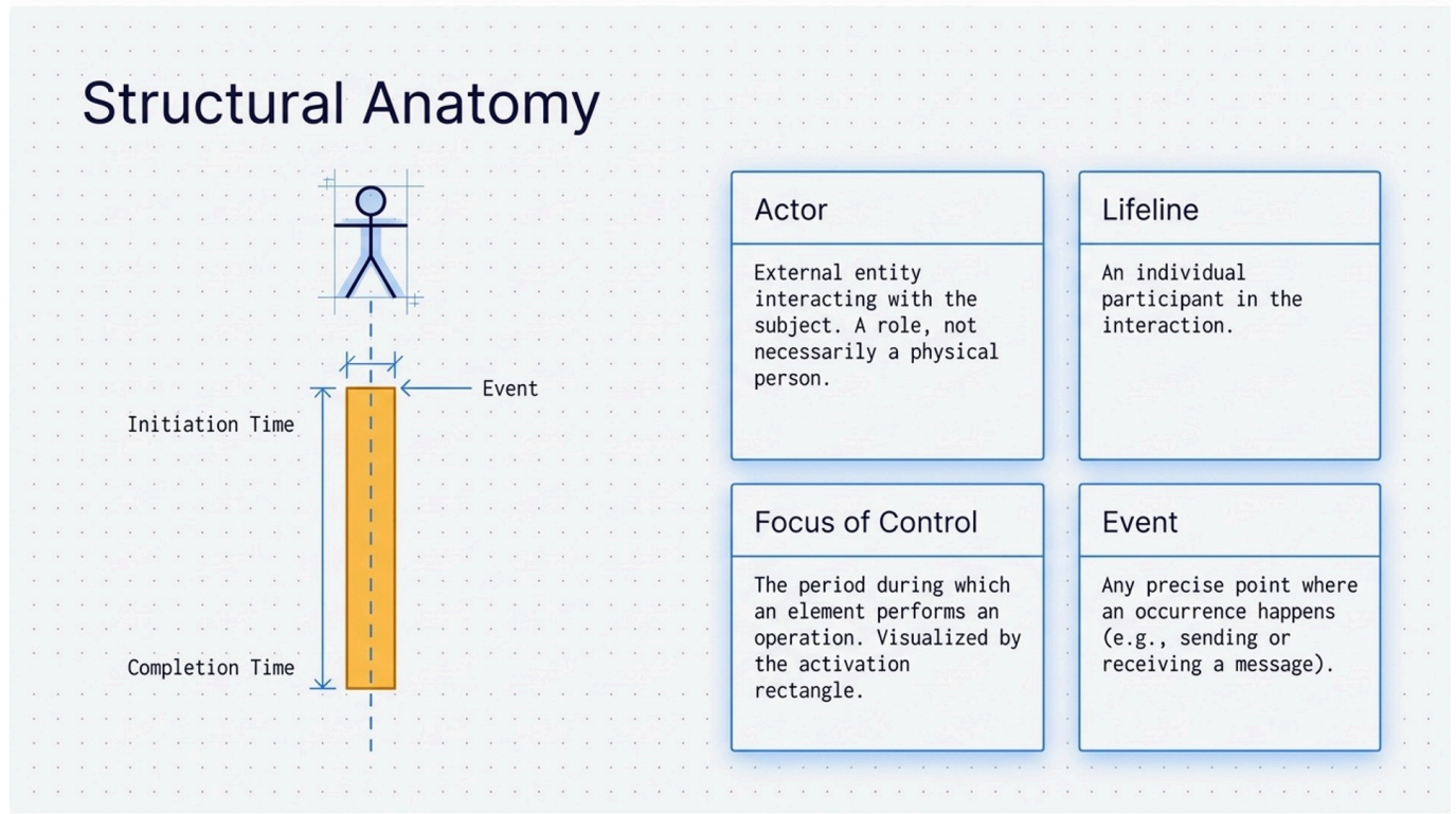
Figure 4.5.3: Lifelines and Activation Focus. The thin vertical rectangle on a lifeline represents the period during which an object is actively executing code or awaiting a subroutine return.
