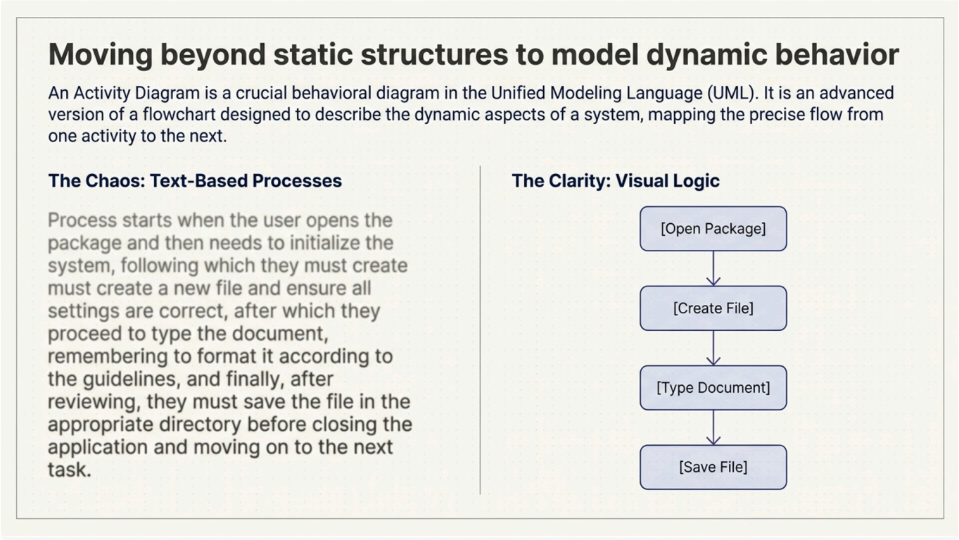
Figure 4.6.1: Visual Logic in Activity Modeling. Activity diagrams extend traditional flowcharts with Petri-net token semantics, parallel fork/join execution, and object state flow.
