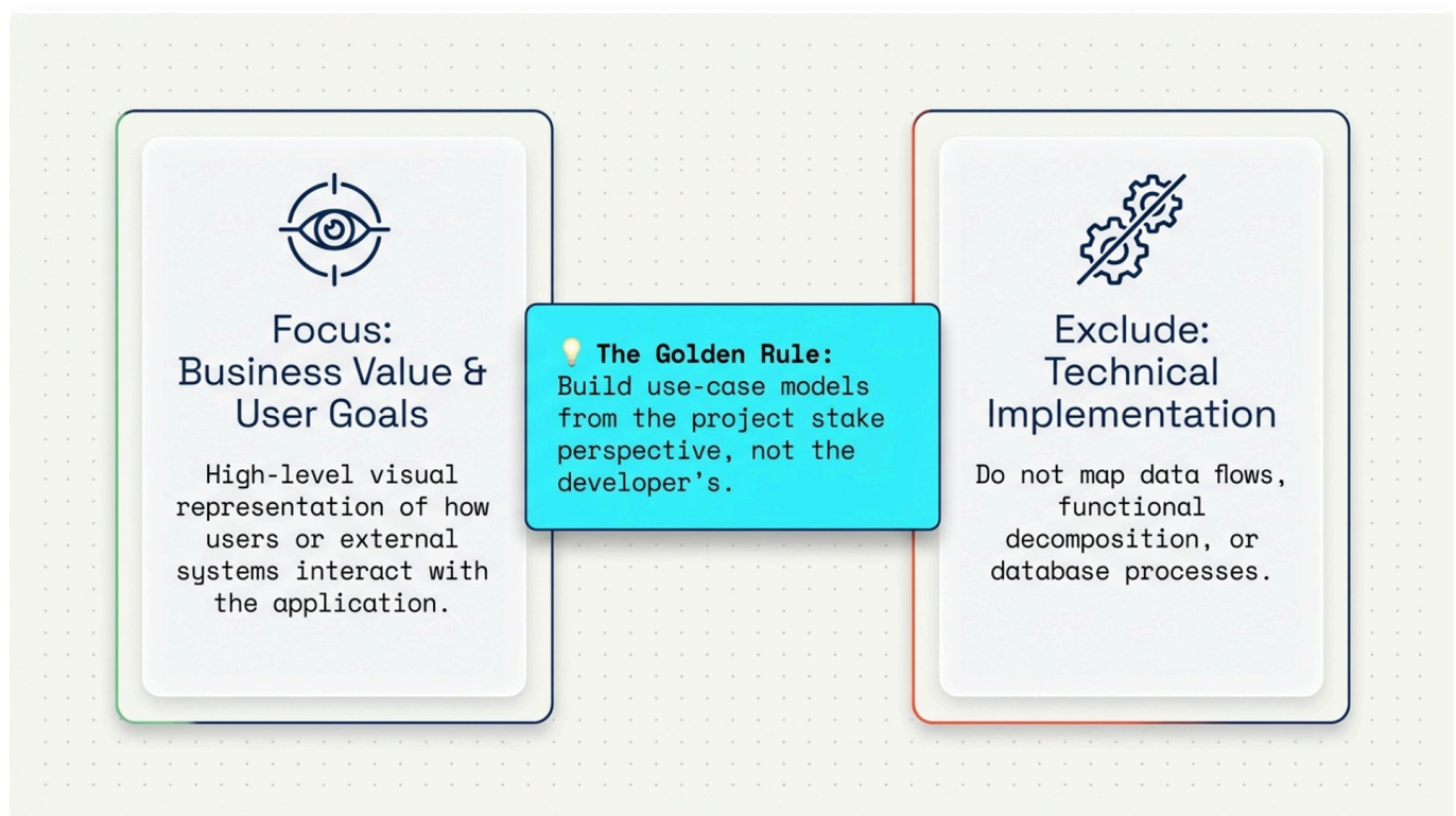
Figure 4.3.2: User Goals vs. Technical Steps. Use cases must represent complete user goals yielding business value, not fine-grained UI clicks or CRUD sub-operations.
