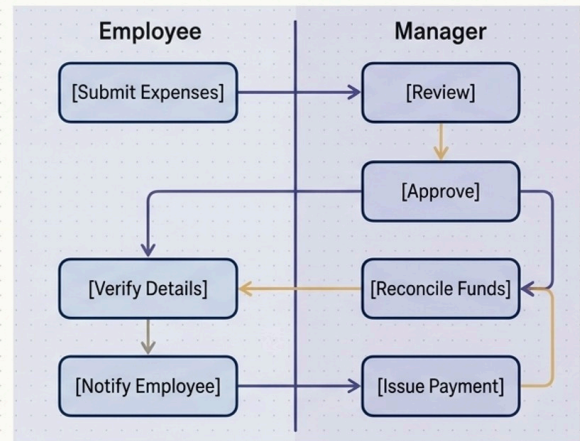
Figure 4.6.4: Swimlanes and Partitions. Columnar divisions allocating responsibility for specific actions to distinct business roles or architectural subsystems.
