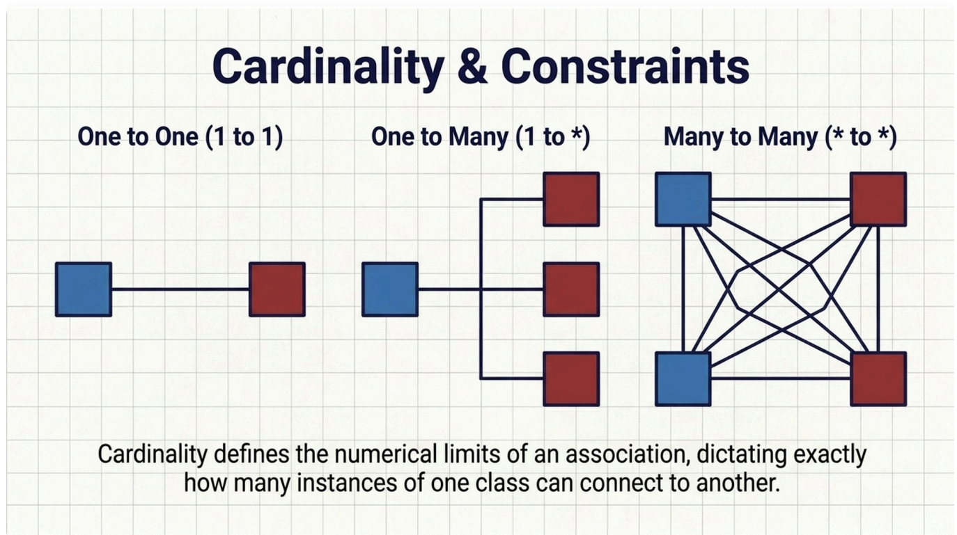
Figure 4.4.7: Multiplicity Constraints and Navigability. Specifying lower and upper bounds (1, , 0..1, 1..) on relationship endpoints.
