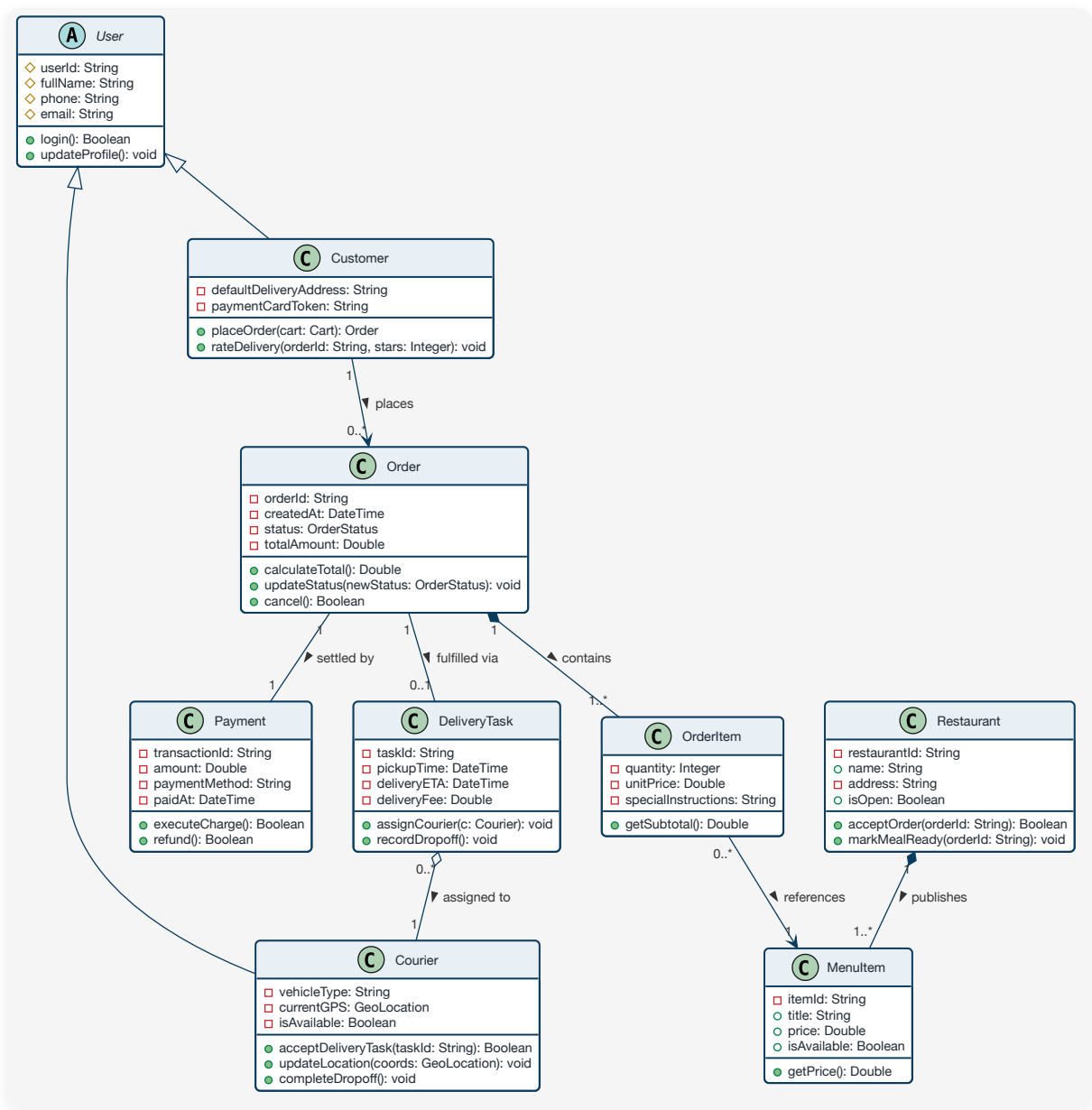
Figure 2.1 QuickBite Platform UML Domain Class Diagram
