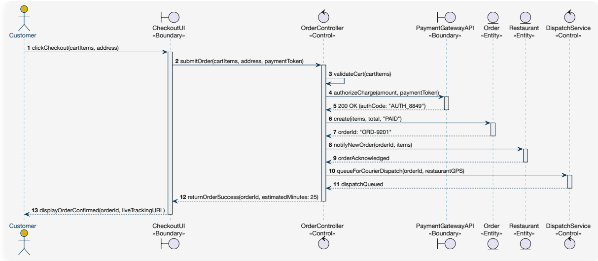
Figure 3.1 QuickBite End-to-End Checkout, Payment & Dispatch Sequence Diagram
