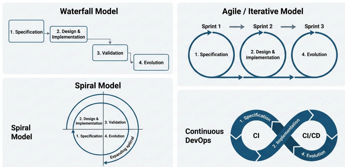
Figure 1.6.3: How the four universal activities (Specification, Design & Implementation, Validation, Evolution) are structured across major software process models—from linear Waterfall cascades and iterative Agile sprint cycles to risk-driven Spiral quadrants and continuous DevOps infinity loops.
