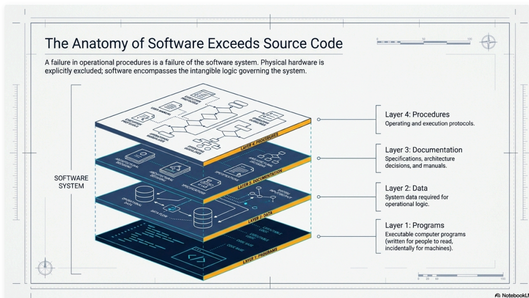
Figure 1.3.1: The IEEE Anatomy of Software—comprising Programs, Data & Schemas, Operational Procedures, and Documentation.
