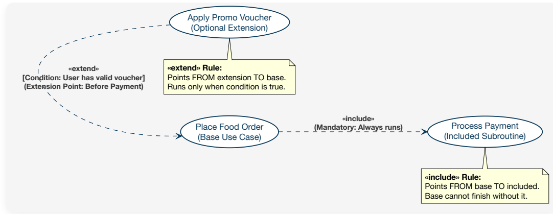
Figure 3.2 Detail of <> and <> Relationships in Order Checkout
