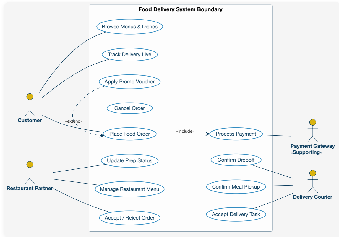
Figure 3.1 QuickBite Comprehensive Use Case Diagram
