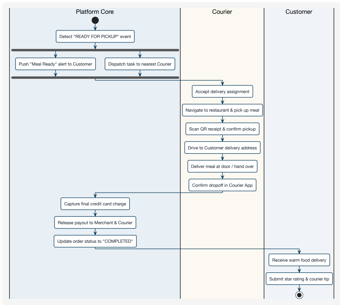
Figure 3.4 Phase 2: Courier Dispatch, Pickup & Delivery Handover Activity Workflow
