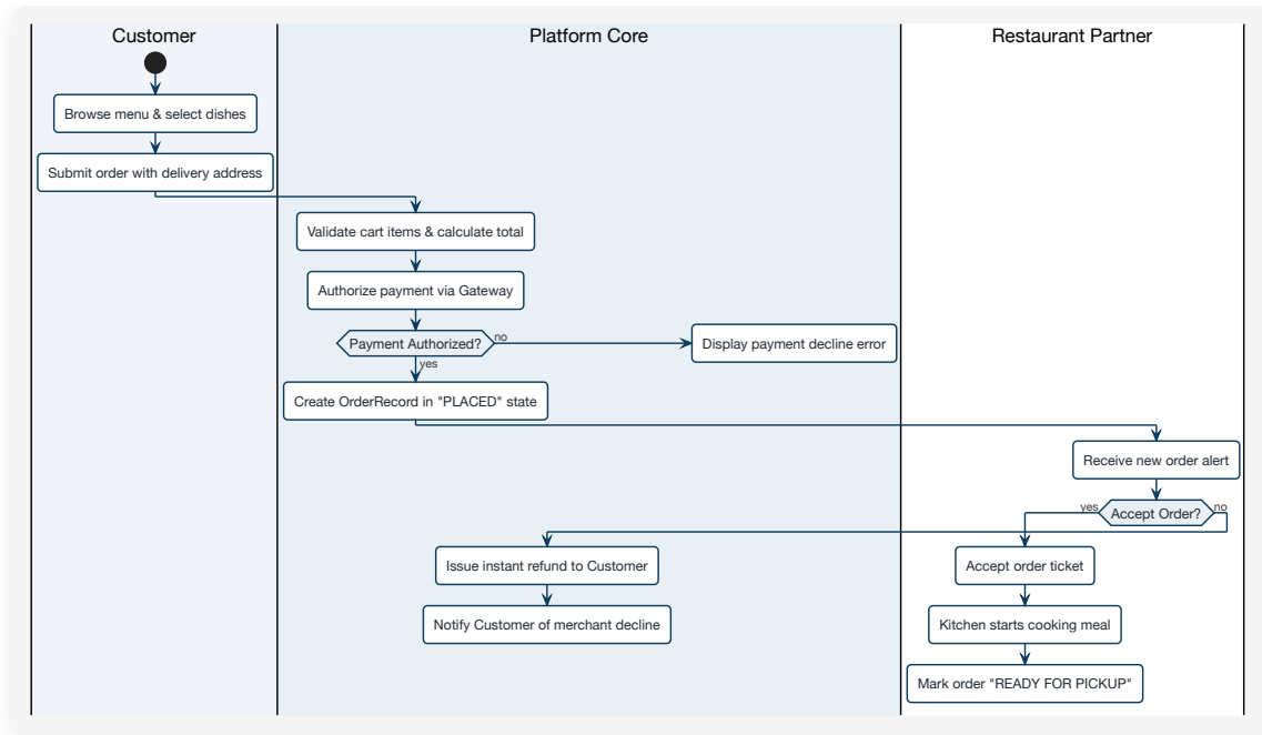
Figure 3.3 Phase 1: Customer Order, Payment Authorization & Kitchen Prep Activity Workflow
