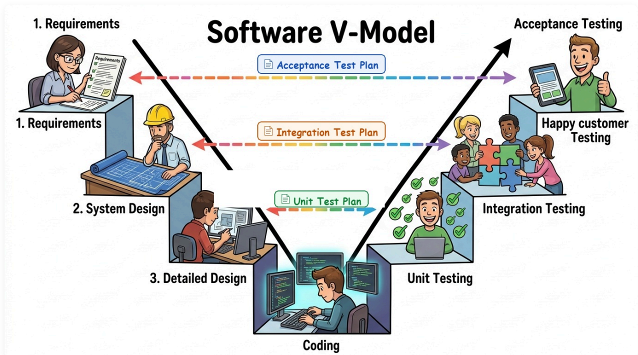
Figure 2.2.2: The V-Model. The left downward arm specifies and decomposes the system; the right upward arm integrates and validates components. Horizontal arrows illustrate that test suites are designed concurrently with specifications.
