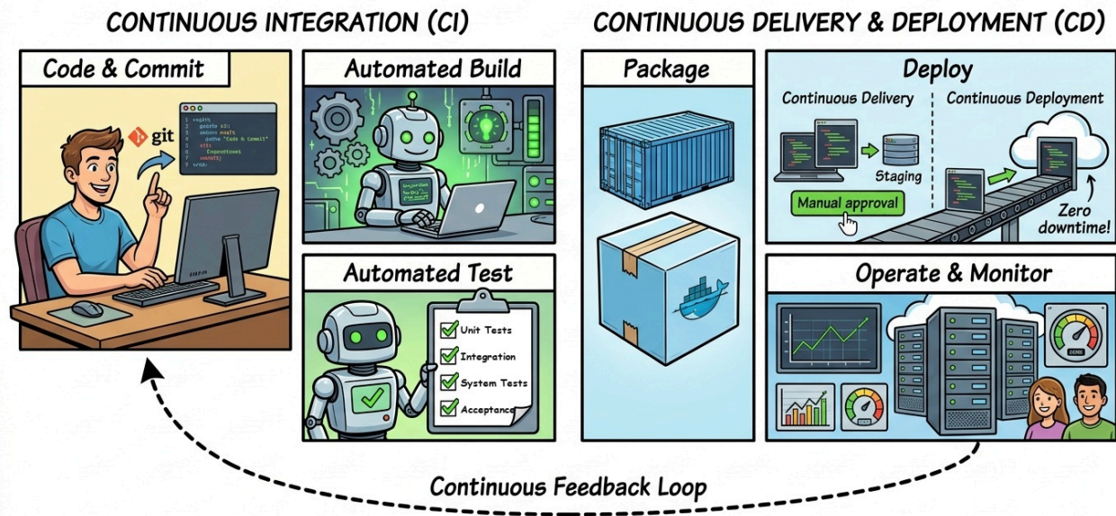
Figure 2.8.2: End-to-End Automated CI/CD Pipeline. From local Git commit to cloud production deployment, automated testing, container packaging, and canary deployments create a smooth, reliable software factory.
