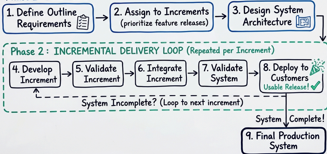
Figure 2.3.1: Incremental Delivery. High-priority functional slices are designed, implemented, tested, and shipped in sequential increments, delivering early business value while establishing an operational baseline.
