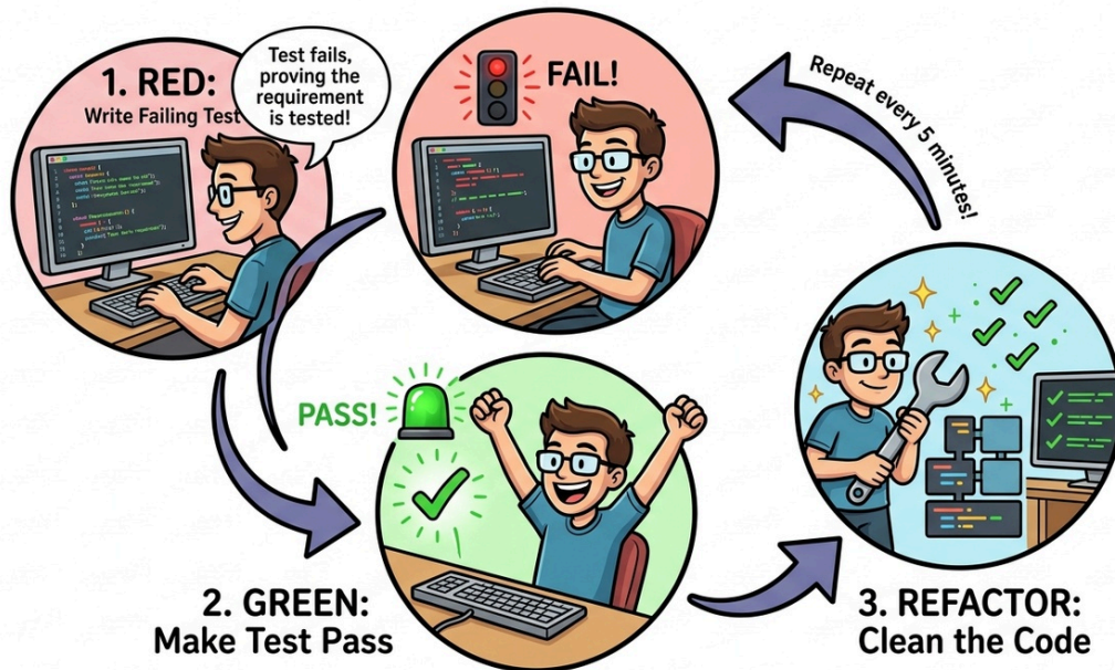
Figure 2.7.3: The TDD Cycle. 1. Red: Write a failing unit test; 2. Green: Make it pass with minimal code; 3. Refactor: Eliminate duplication and improve structure while all tests stay green.
