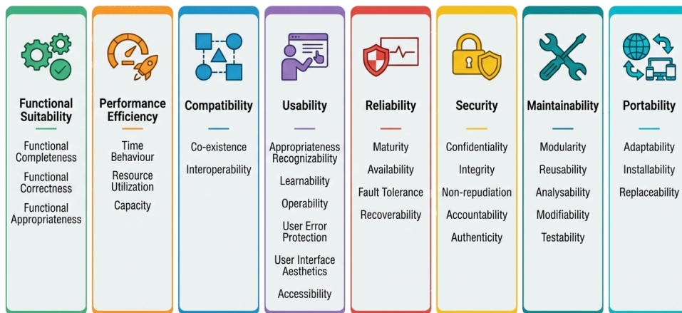
Figure 1.6.1: The ISO/IEC 25010 Product Quality Model—defining 8 core characteristics and their sub-attributes.
