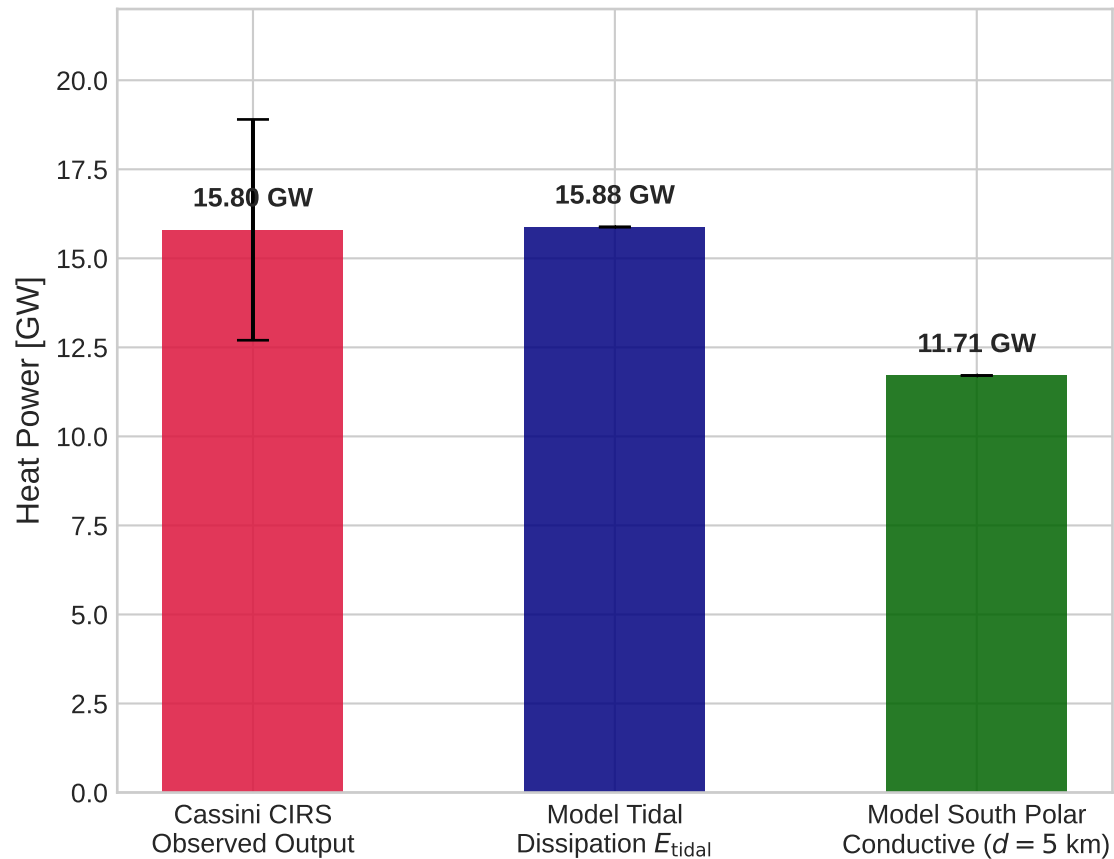
Cassini CIRS Observations vs Tidal Model
