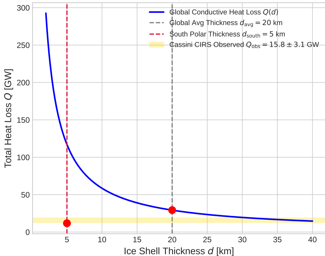
Conductive Heat Transport vs Shell Thickness
