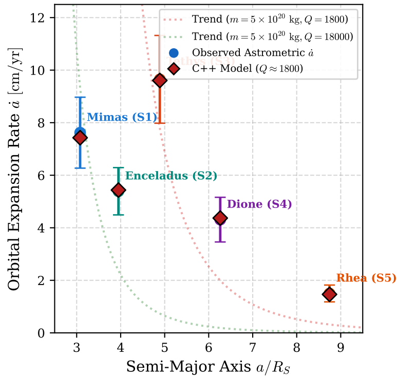
(b) Moon Recession Rates \dot{a} vs Distance
