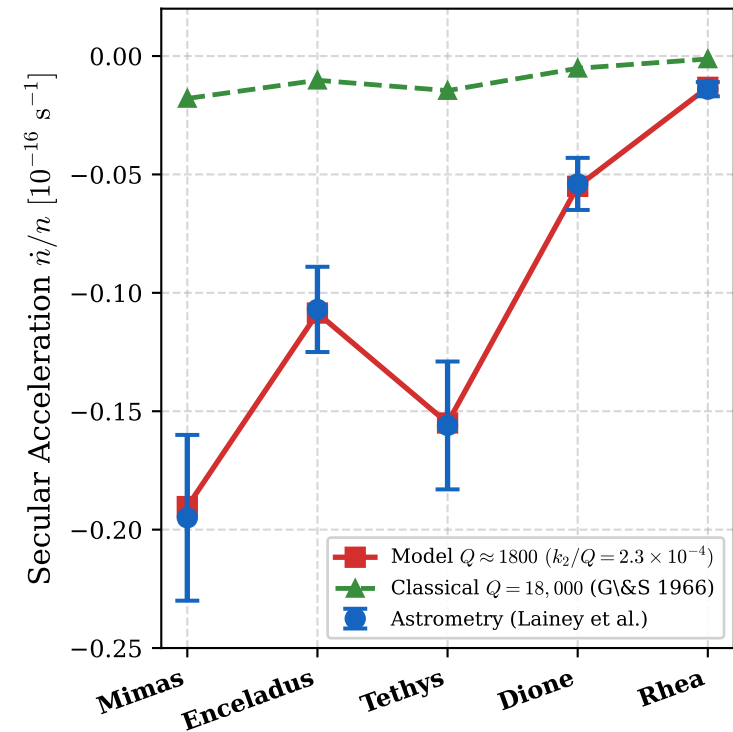
(a) Astrometric Secular Acceleration \dot{n}/n
