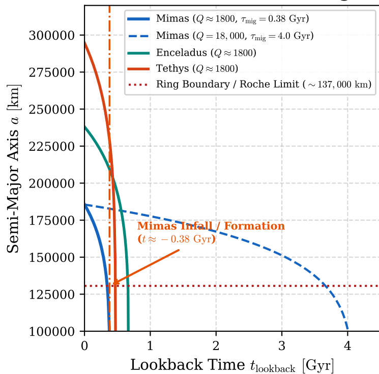
(b) Backward Orbital Evolution & Age Paradox
