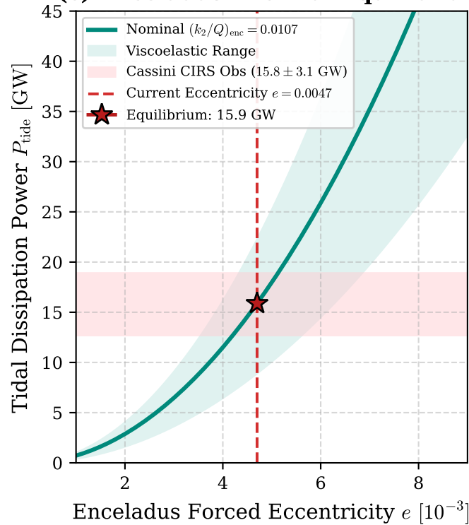
(c) Enceladus Thermal Equilibrium
