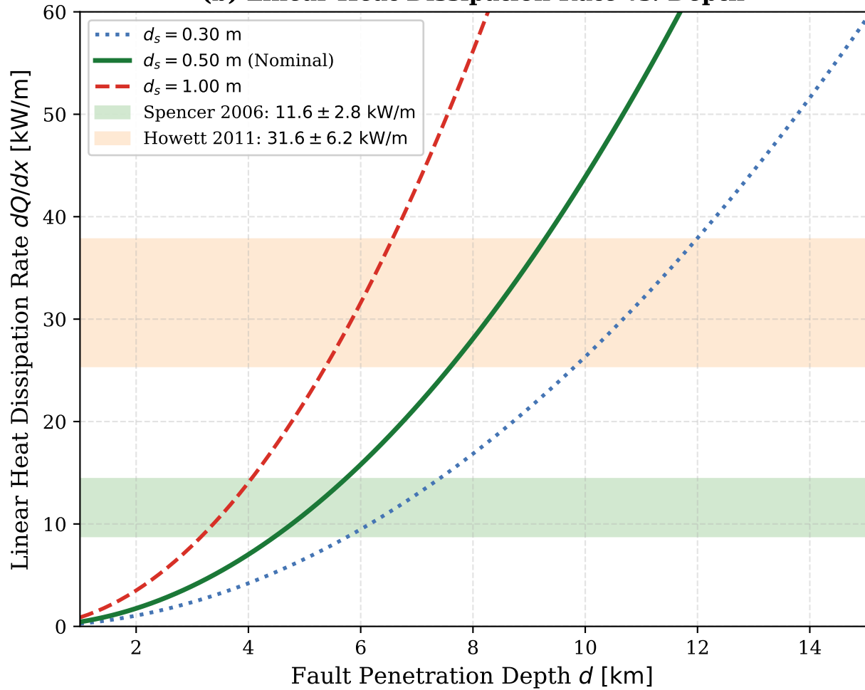
(b) Linear Heat Dissipation Rate vs. Depth
