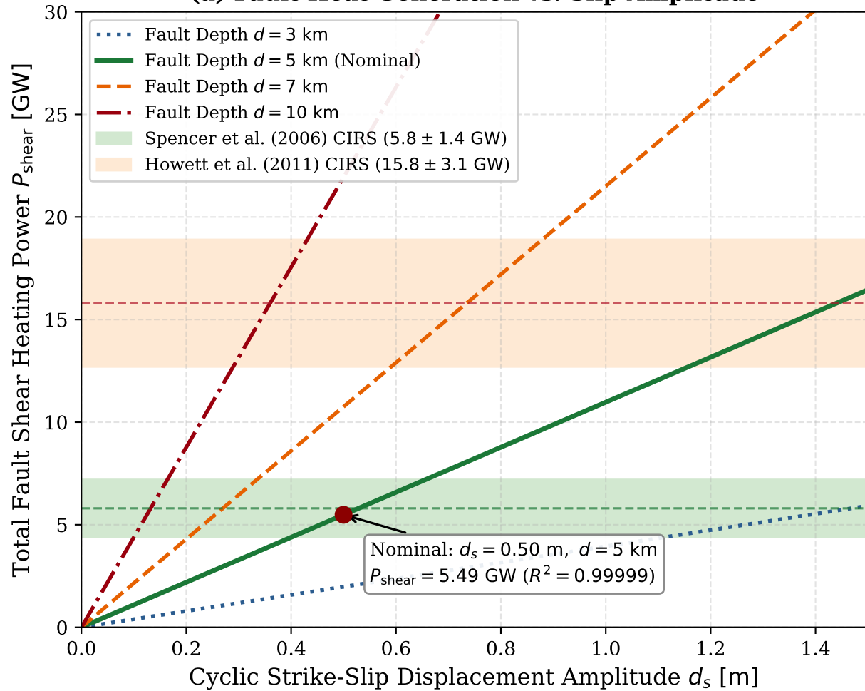
(a) Fault Heat Generation vs. Slip Amplitude
