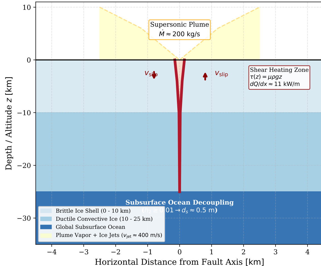
(b) Tiger Stripe Cross-Section & Plume Venting
