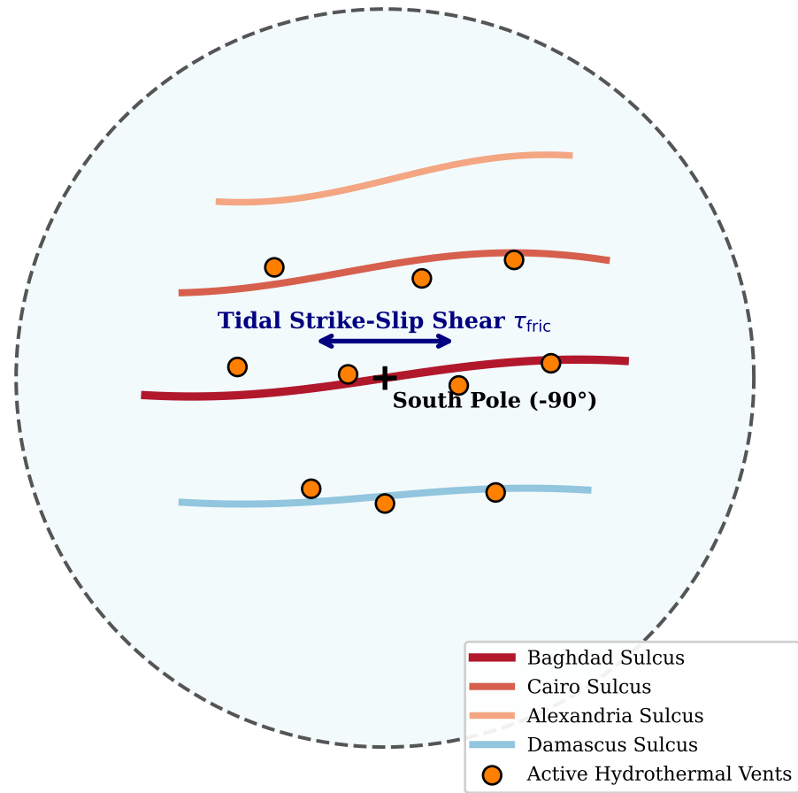
(a) South Polar Terrain (SPT) Tiger Stripes
