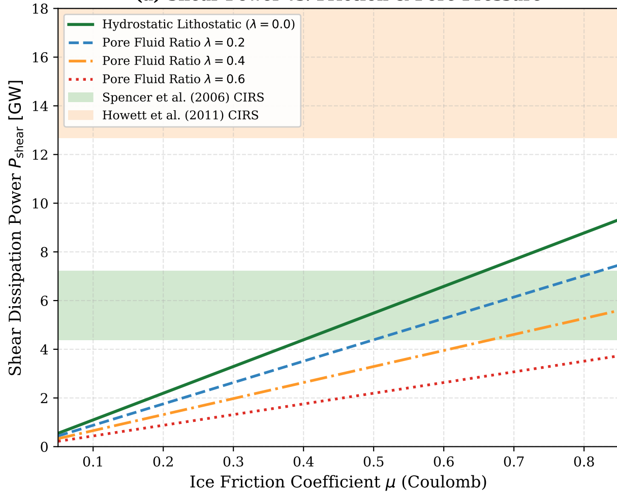
(a) Shear Power vs. Friction & Pore Pressure
