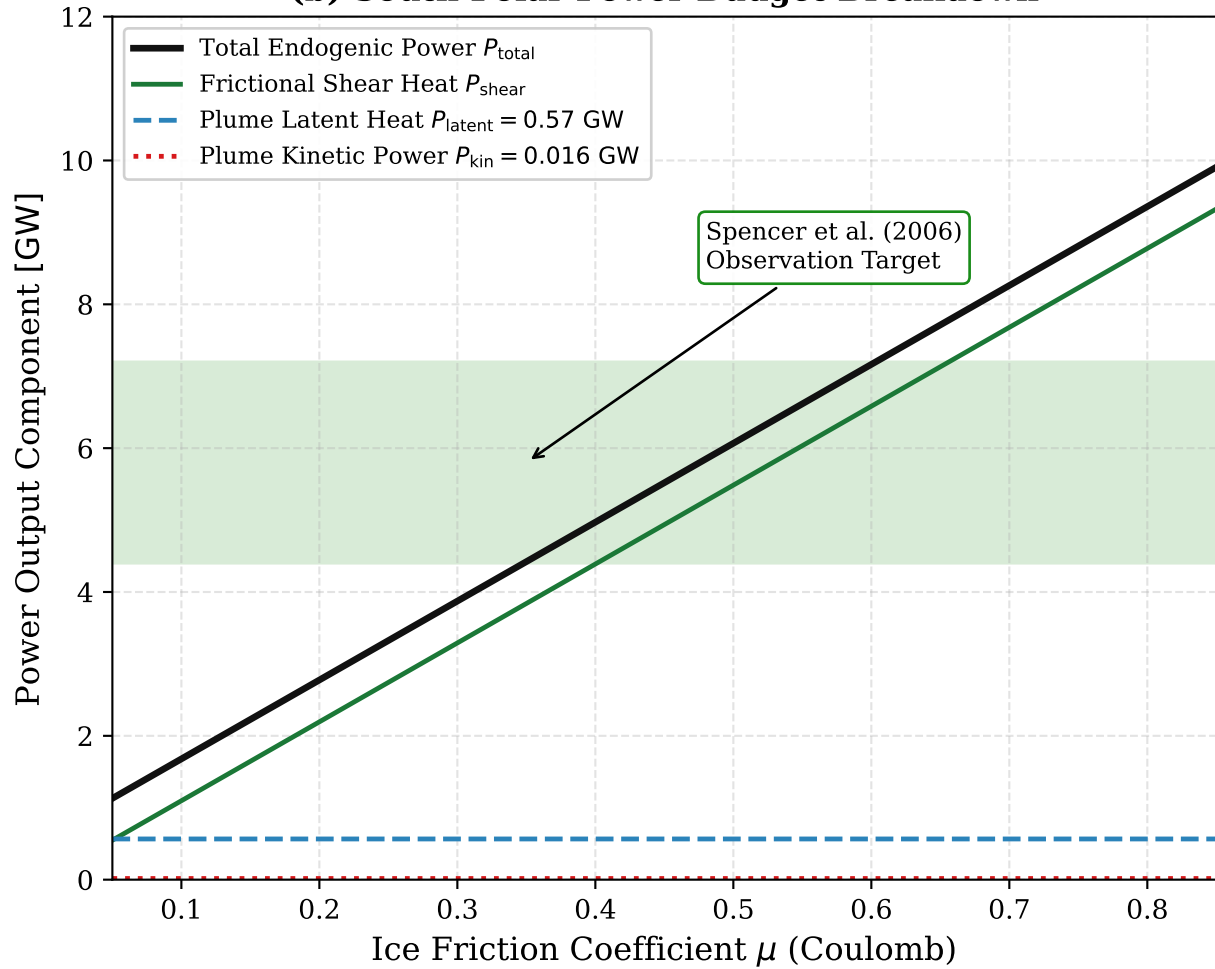
(b) South Polar Power Budget Breakdown
