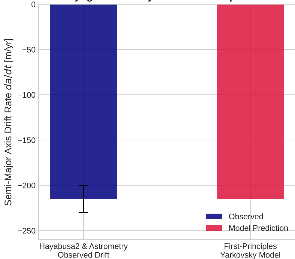
Ryugu Yarkovsky Drift Rate Comparison
