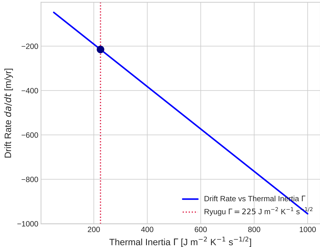
Model Choice: Sensitivity to Thermal Inertia
