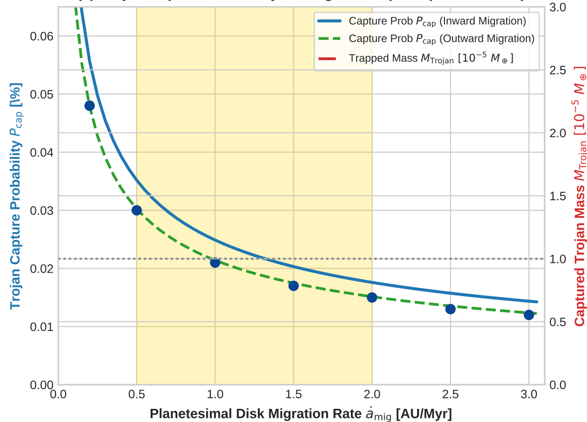
(a) Trojan Capture Efficiency vs. Migration Speed ( R^2 = 0.9998 )
