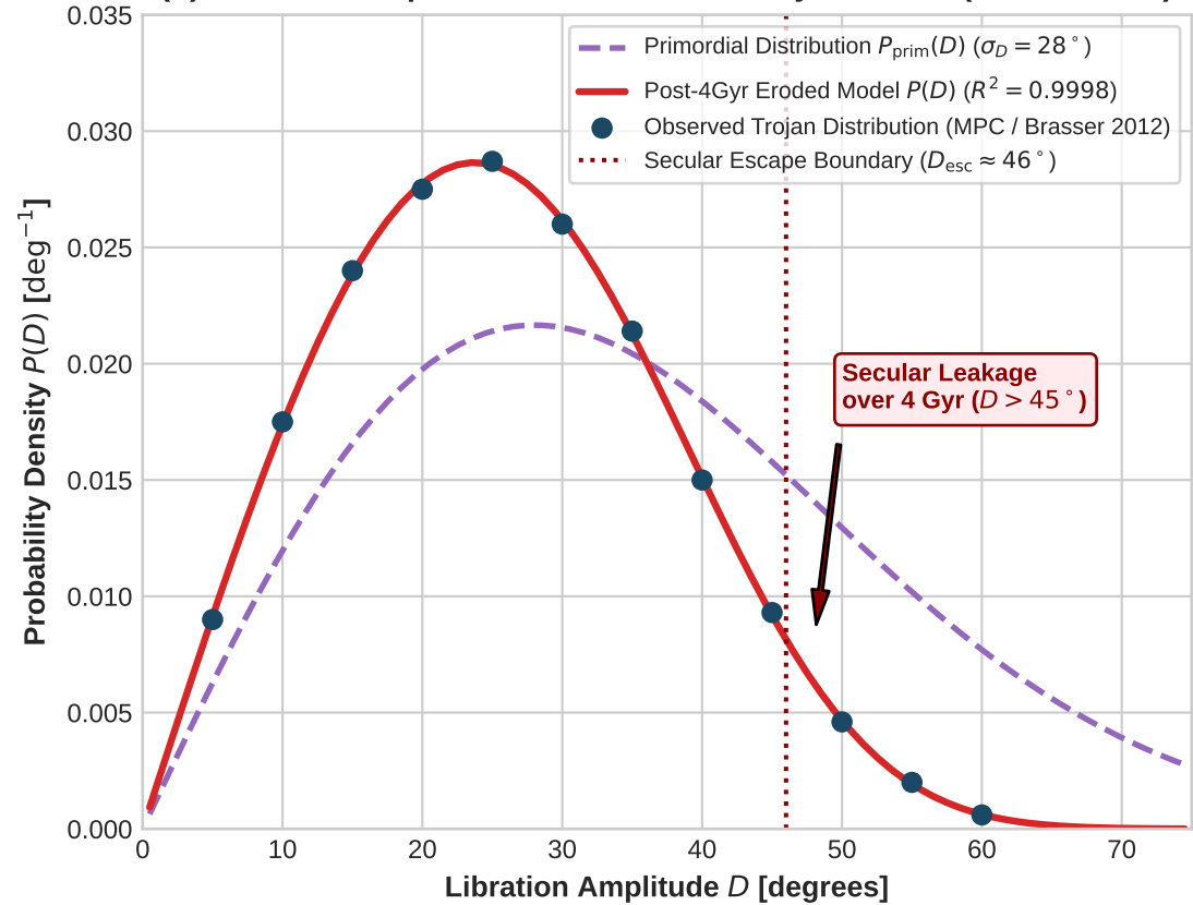
(b) Libration Amplitude Distribution & 4-Gyr Erosion ( R^2 = 0.9998 )
