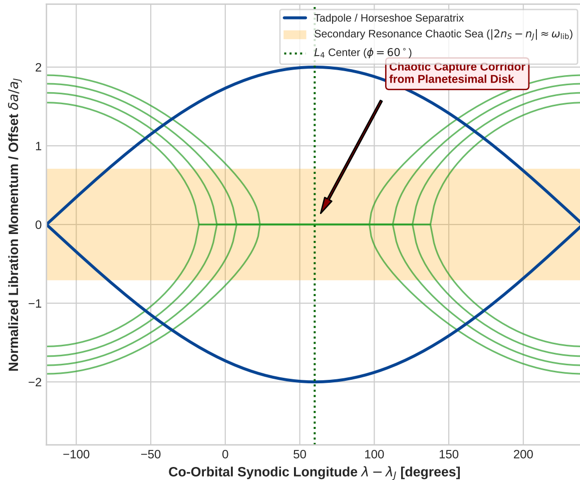
(b) Phase Space Libration Topology & Chaotic Capture
