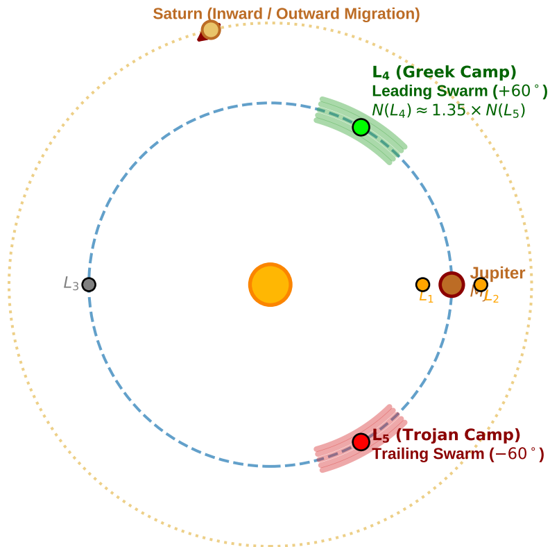
(a) Co-Orbital Lagrangian Geometry & Trojan Swarms
