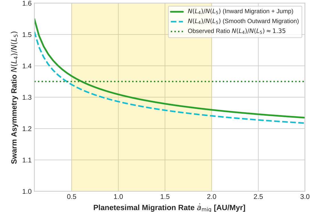
(c) Leading vs. Trailing Swarm Asymmetry N(L_4)/N(L_5)
