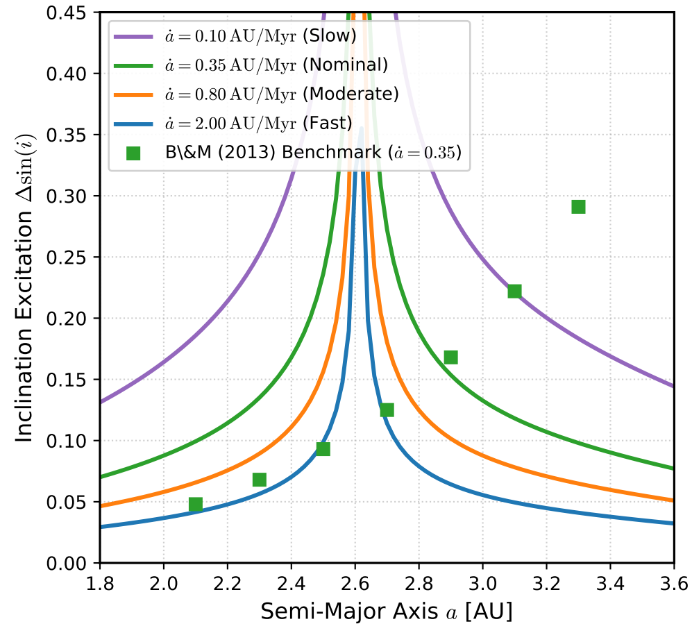
(b) Analytical Inclination Kick \Delta \sin(i)
