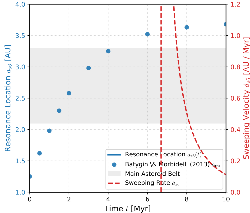
(a) s_6 Secular Resonance Sweeping Rate
