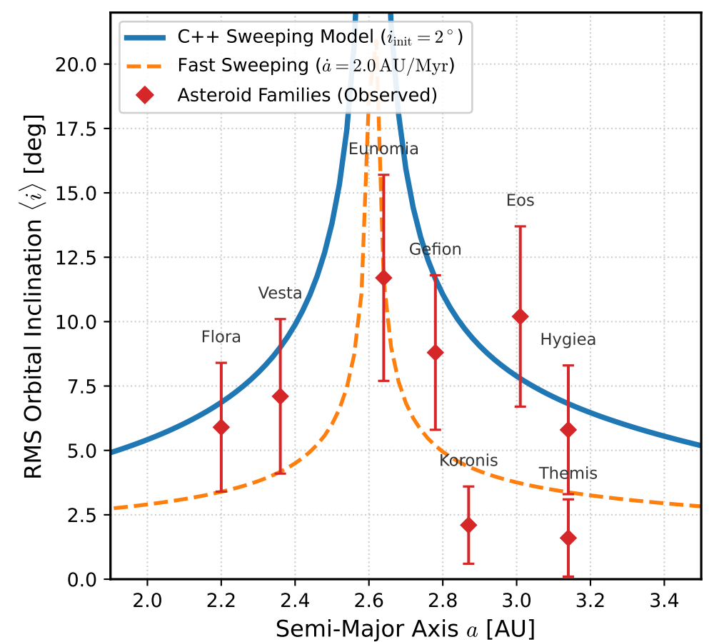
(c) Post-Crossing Inclination vs Asteroid Families
