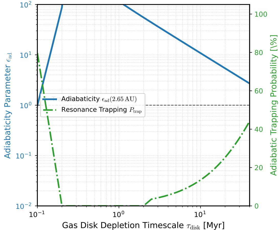
(b) Adiabaticity \epsilon_{\text{ad}} vs Disk Timescale \tau
