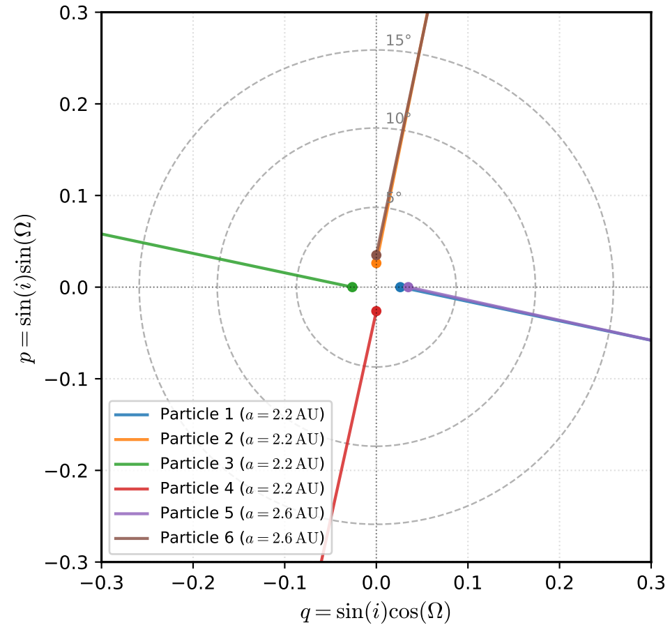
(a) Resonant Phase Space (q, p) Trajectories
