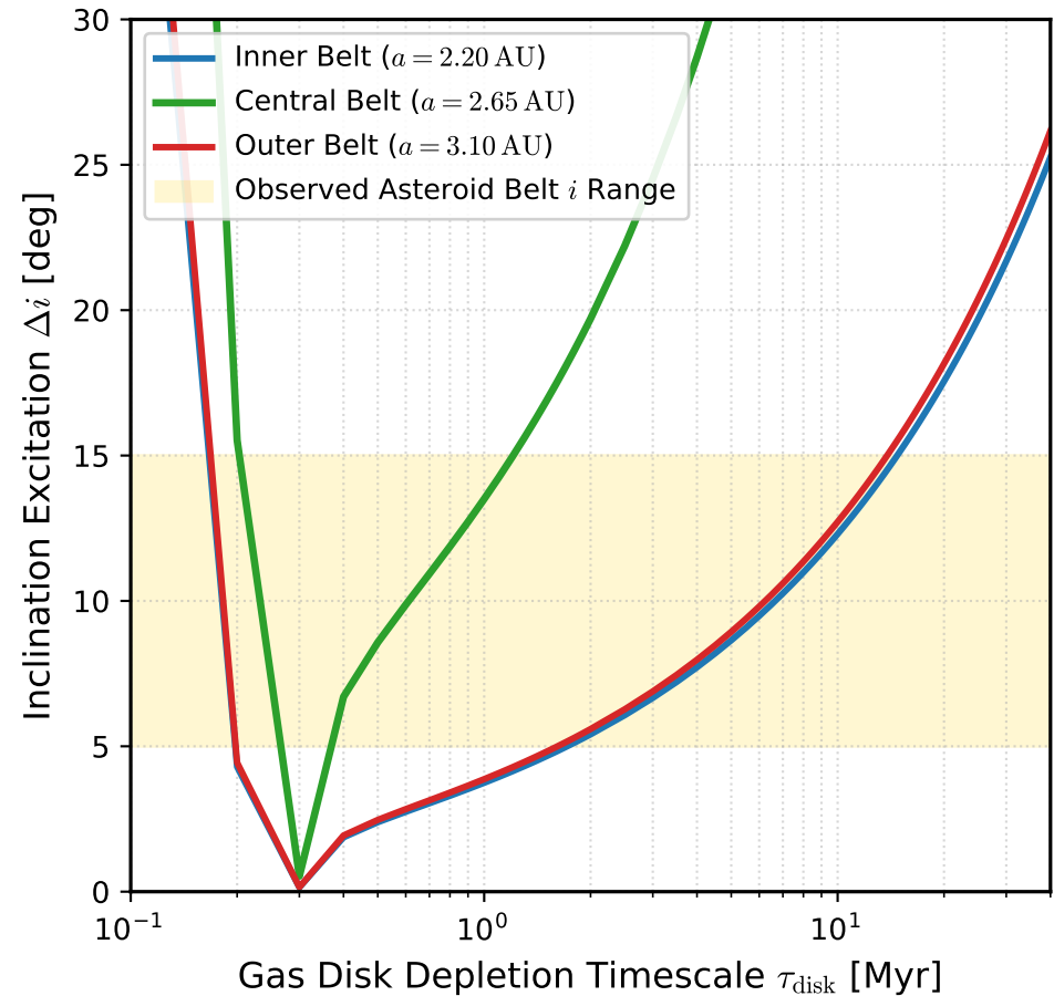
(c) \Delta i Scaling with Gas Dispersal \tau_{\text{disk}}
