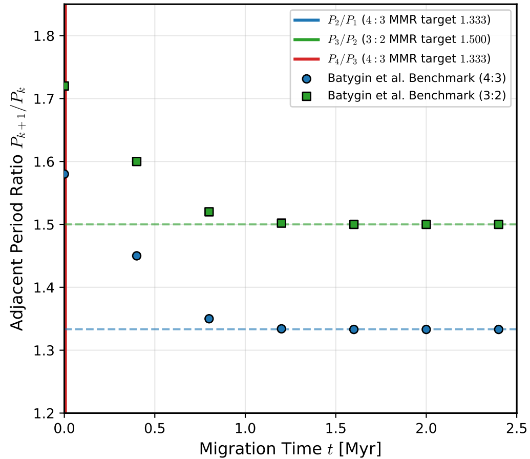
(a) Resonant Chain Locking ( R^2 = 1.000 )
