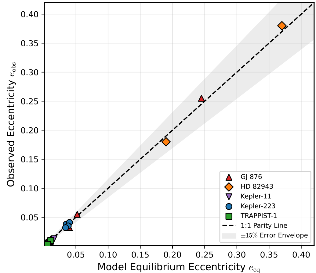
(c) Exoplanet Catalog Match ( R^2 = 0.9976 )
