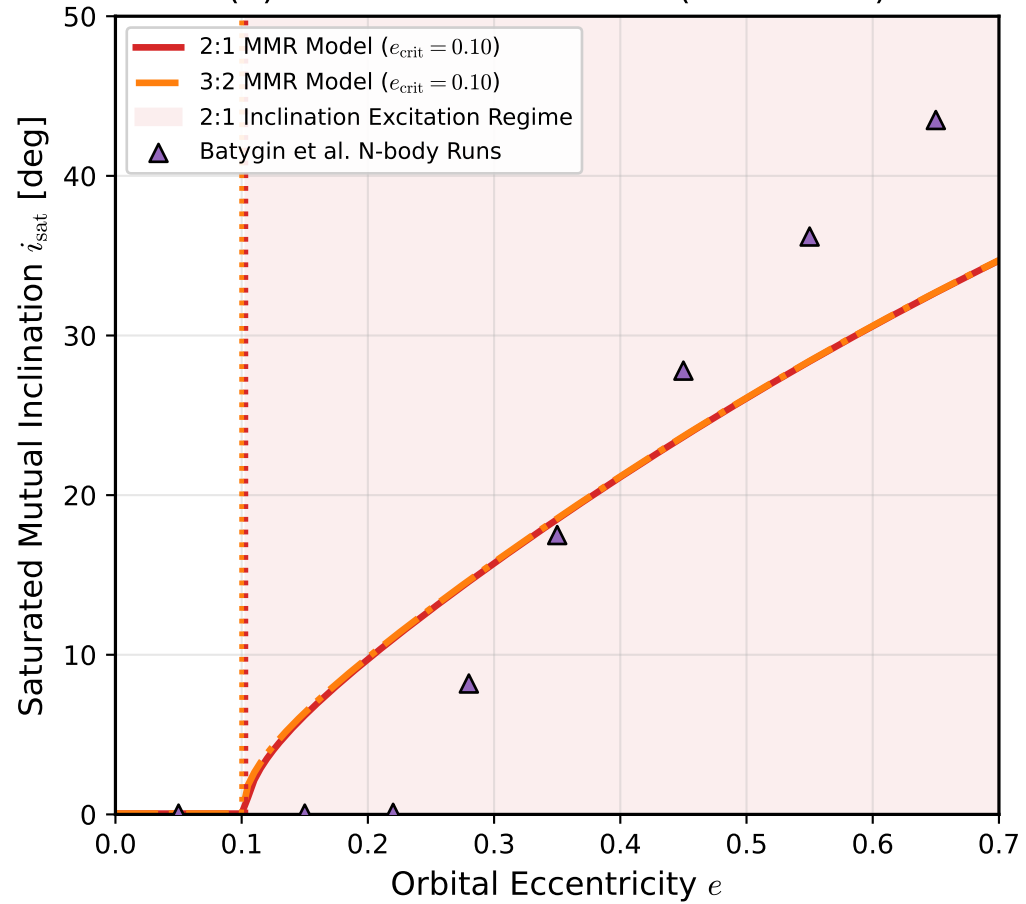
(b) Inclination Bifurcation ( R^2 = 0.9999 )
