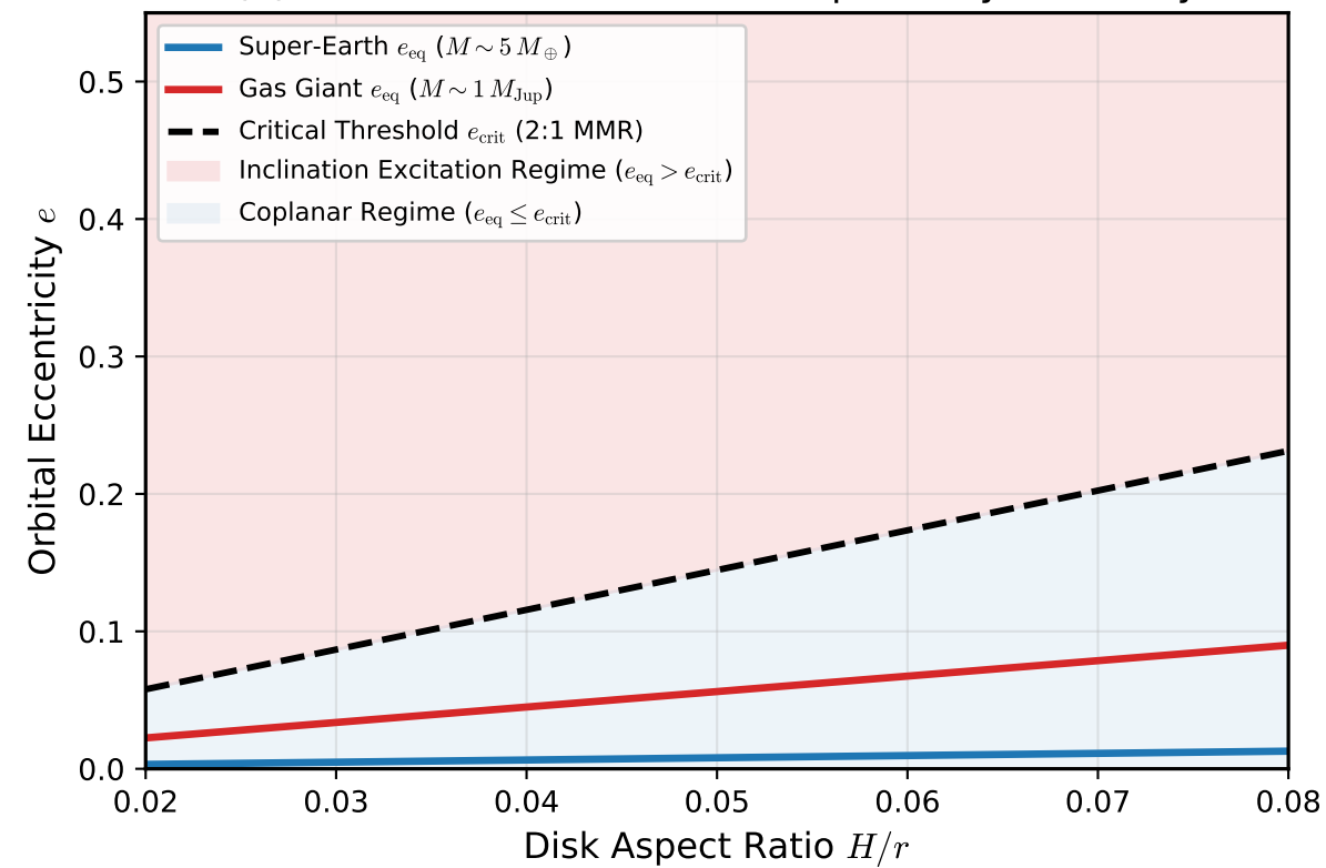
(b) Resonance Excitation vs Coplanarity Boundary
