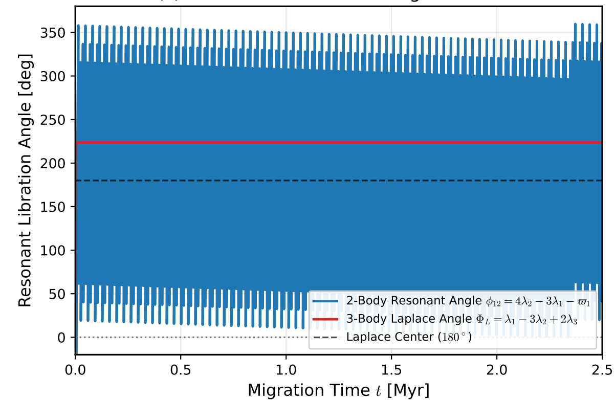
(c) Multi-Planet Resonant Angle Libration
