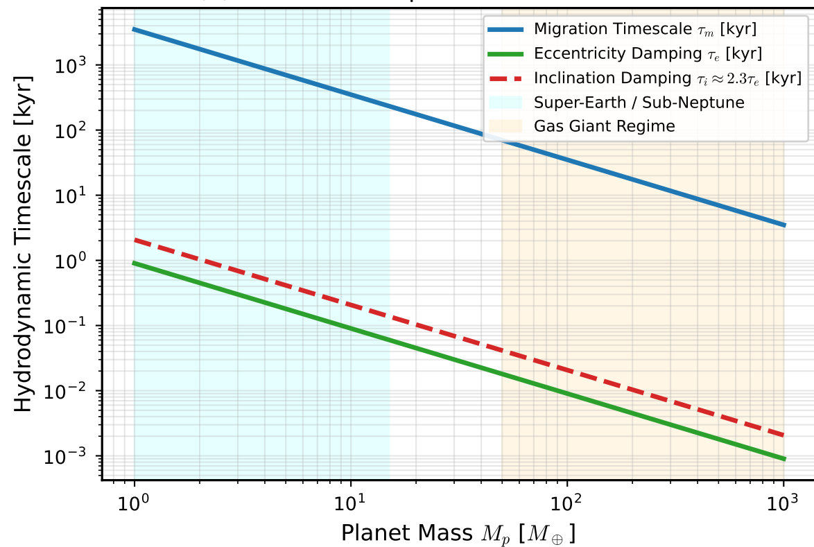
(a) Gas Disk Dissipative Timescales at 1 AU
