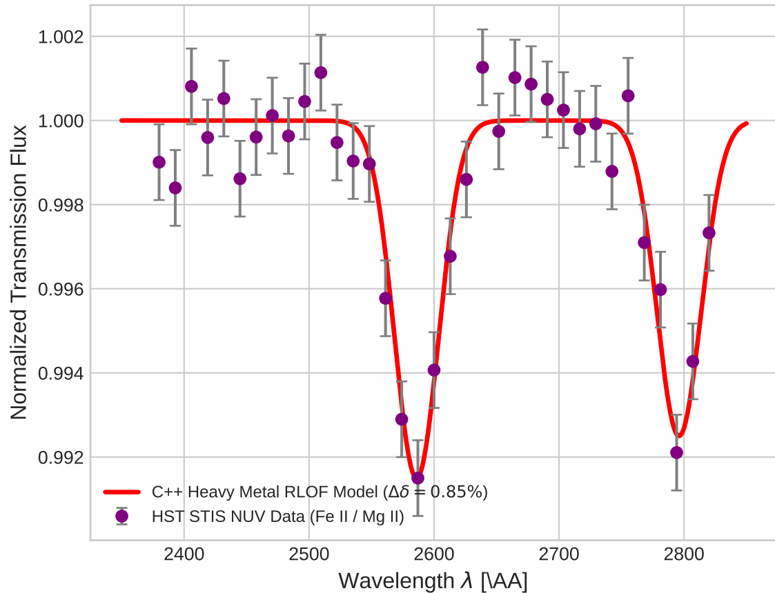
WASP-121b NUV Heavy Metal Transmission
