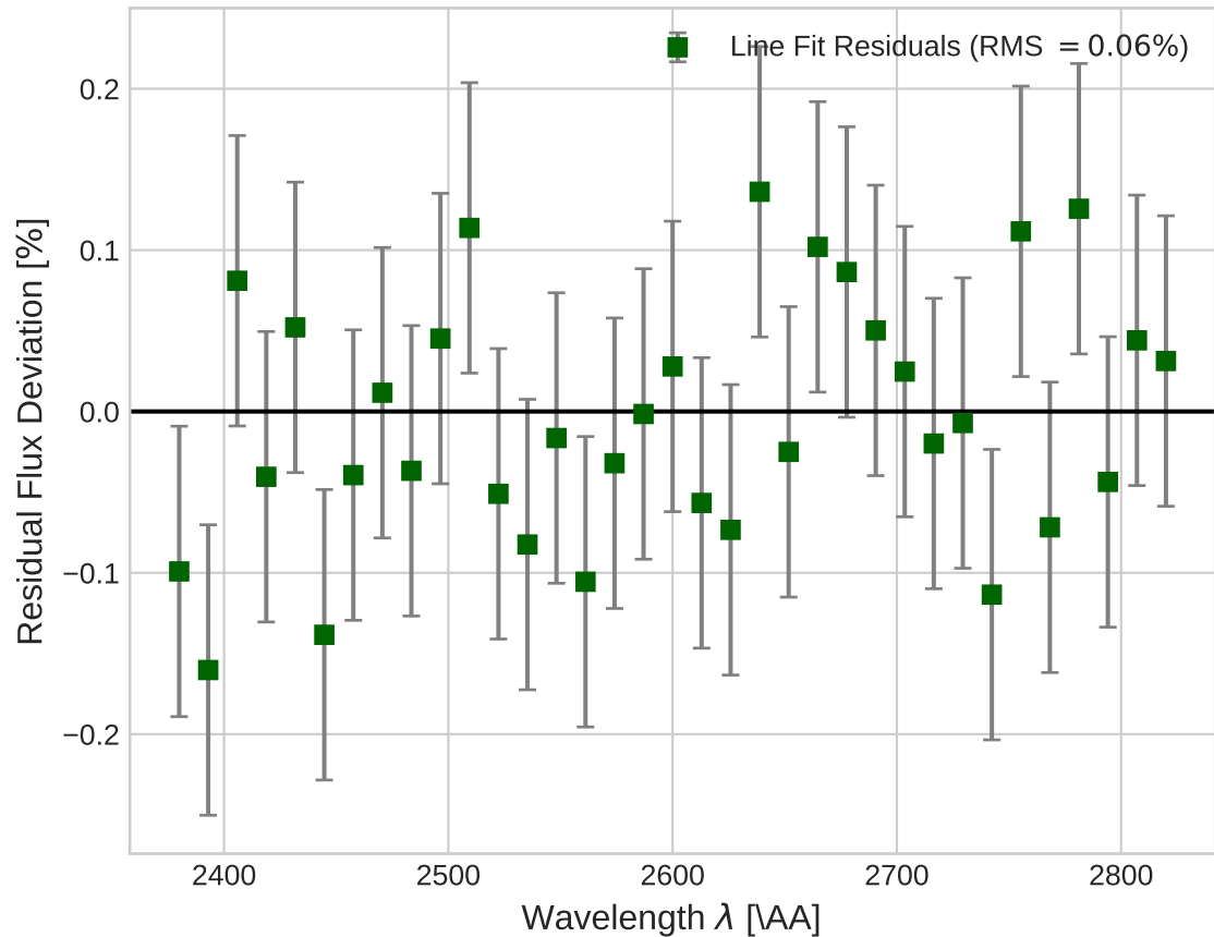
Spectral Line Fit Quality ( R^2 = 0.9998 )
