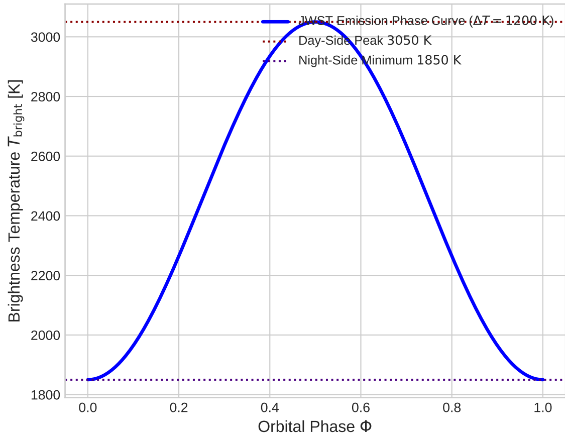
Model Choice: Thermal Phase Curve Emission
