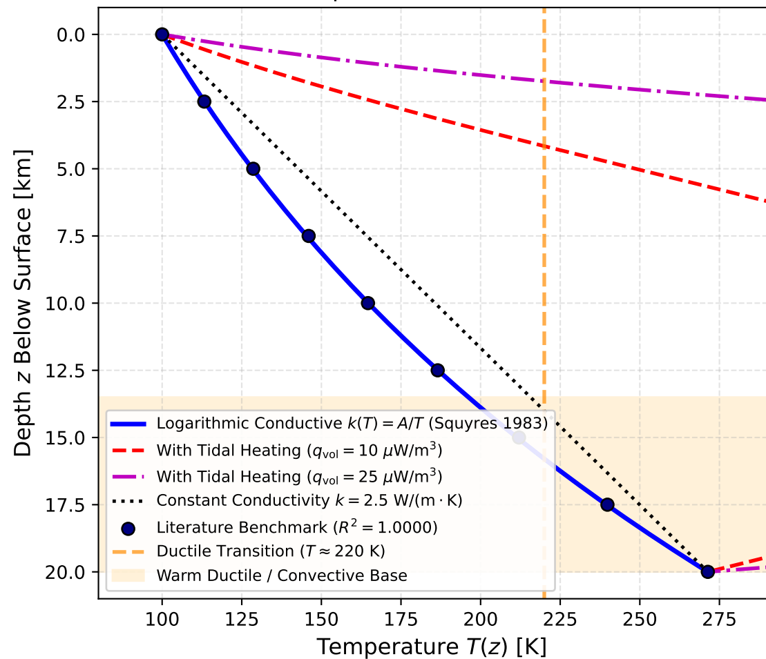
(a) Ice Shell Temperature Profiles T(z) ( H = 20 km)
