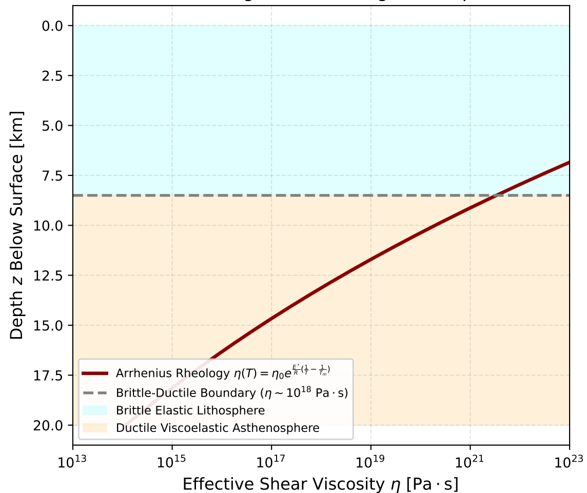
(b) Rheological Weakening with Depth
