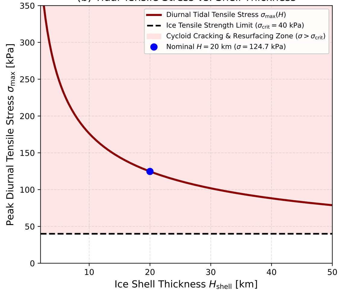
(b) Tidal Tensile Stress vs. Shell Thickness
